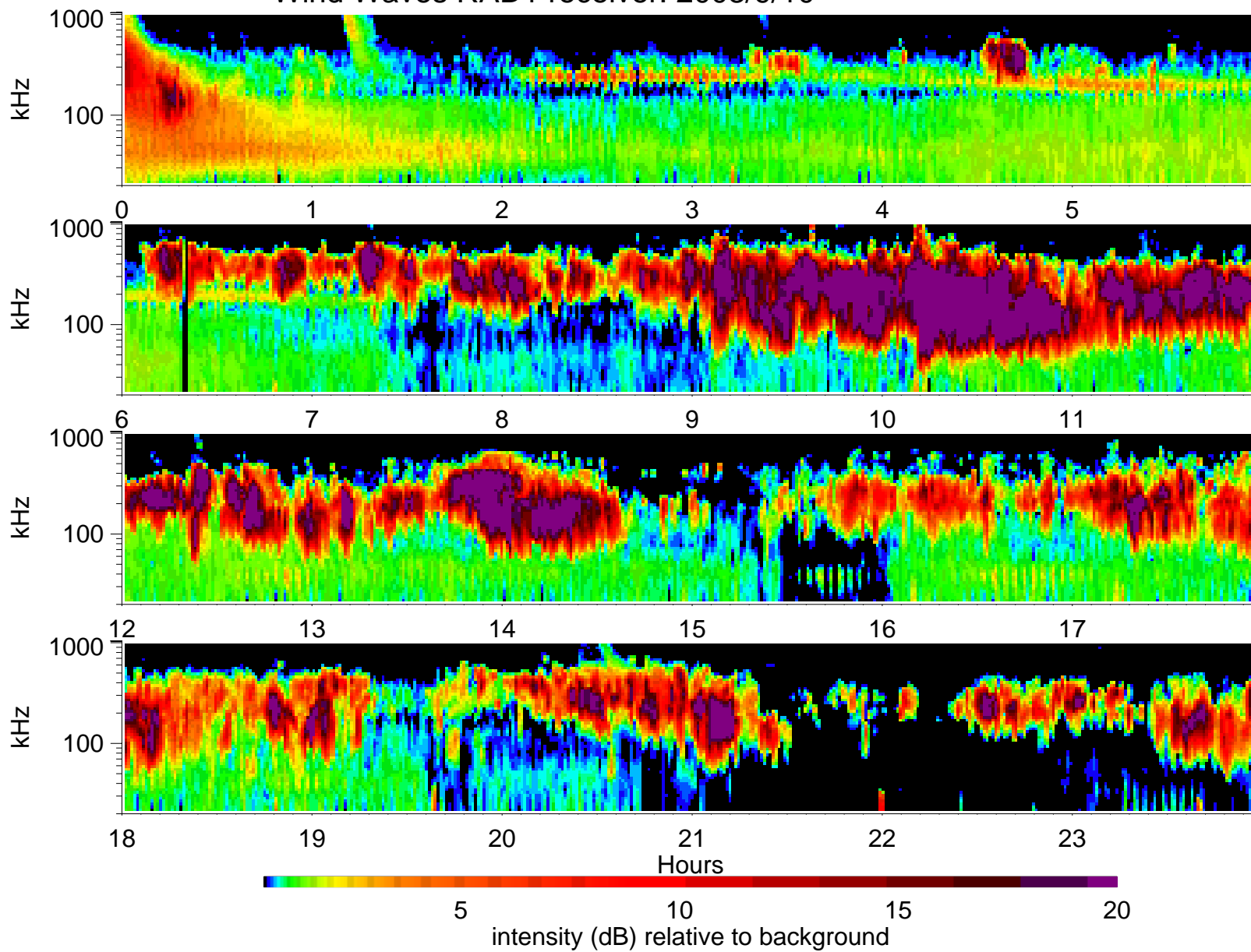
Wind Waves RAD1 receiver: 2003/9/10
