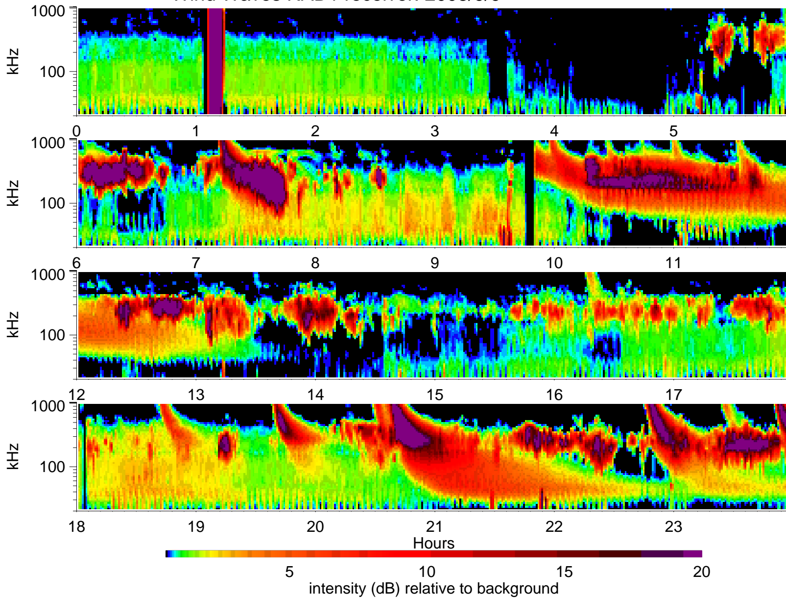
Wind Waves RAD1 receiver: 2003/9/9
