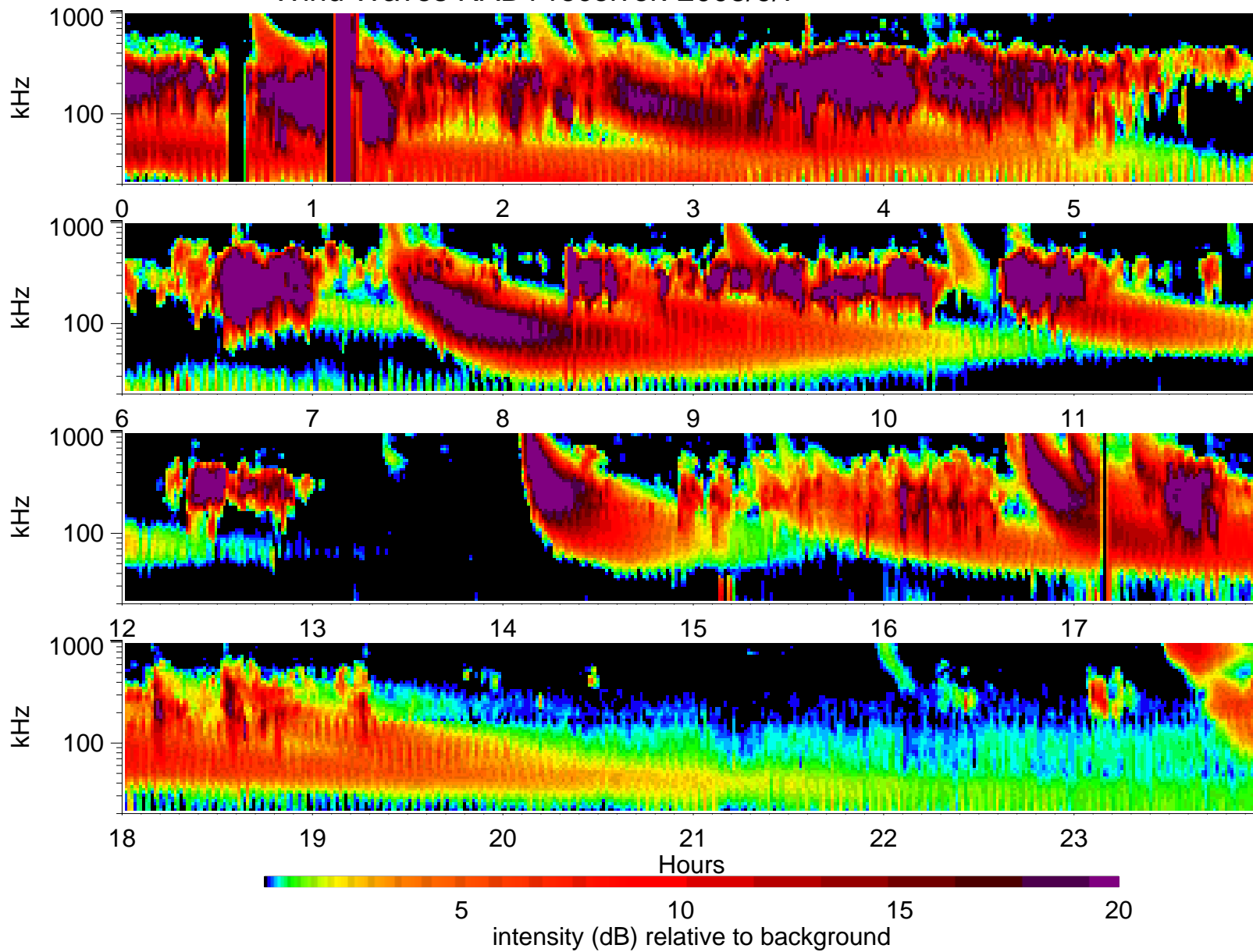
Wind Waves RAD1 receiver: 2003/9/7
