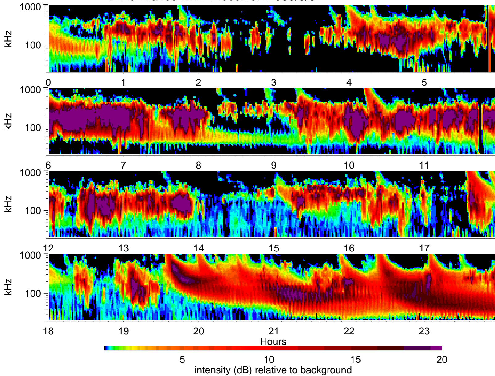
Wind Waves RAD1 receiver: 2003/9/6
