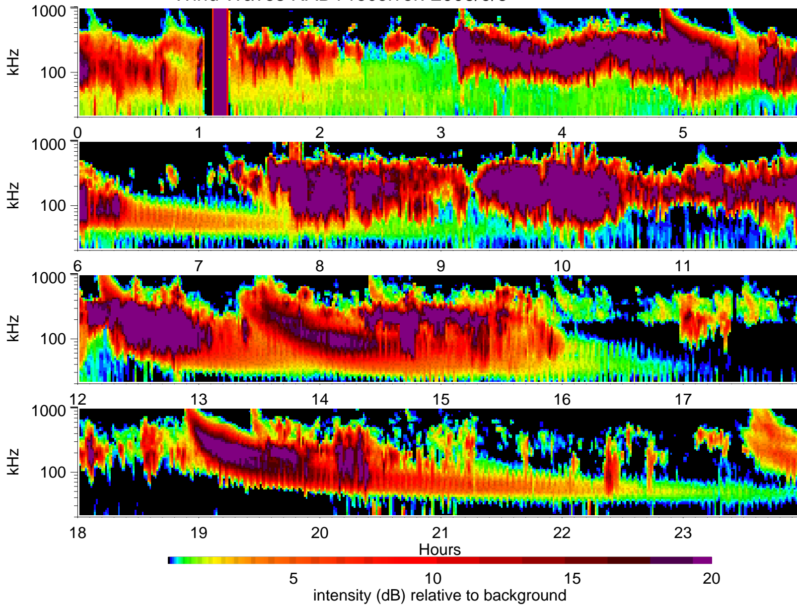
Wind Waves RAD1 receiver: 2003/9/5
