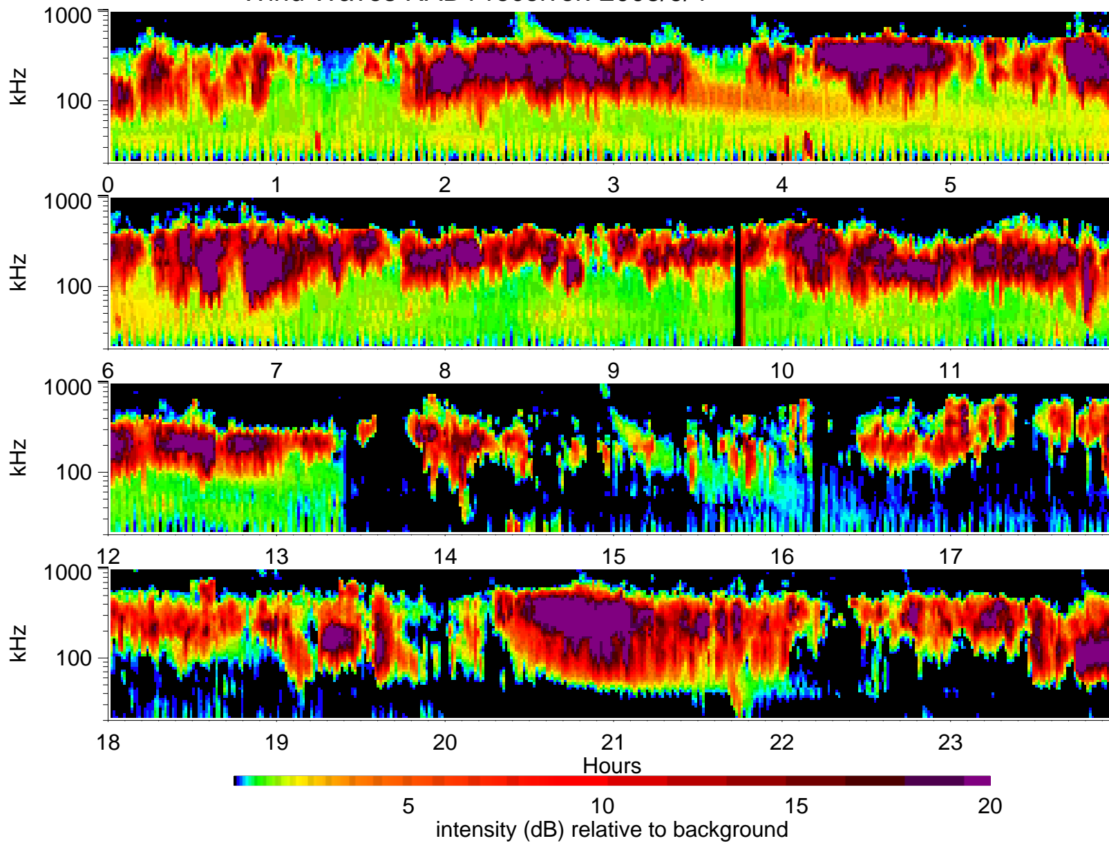
Wind Waves RAD1 receiver: 2003/9/4
