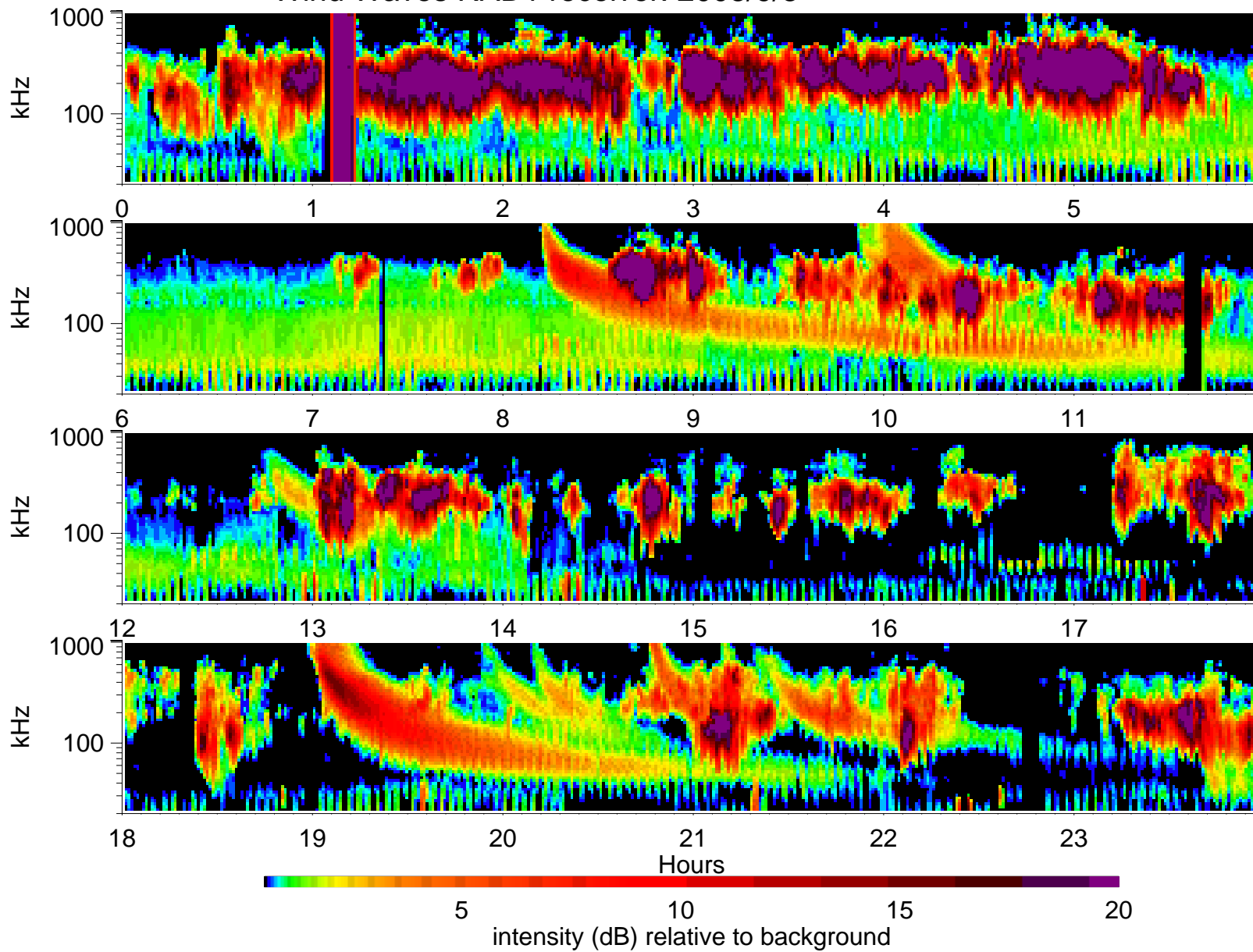
Wind Waves RAD1 receiver: 2003/9/3
