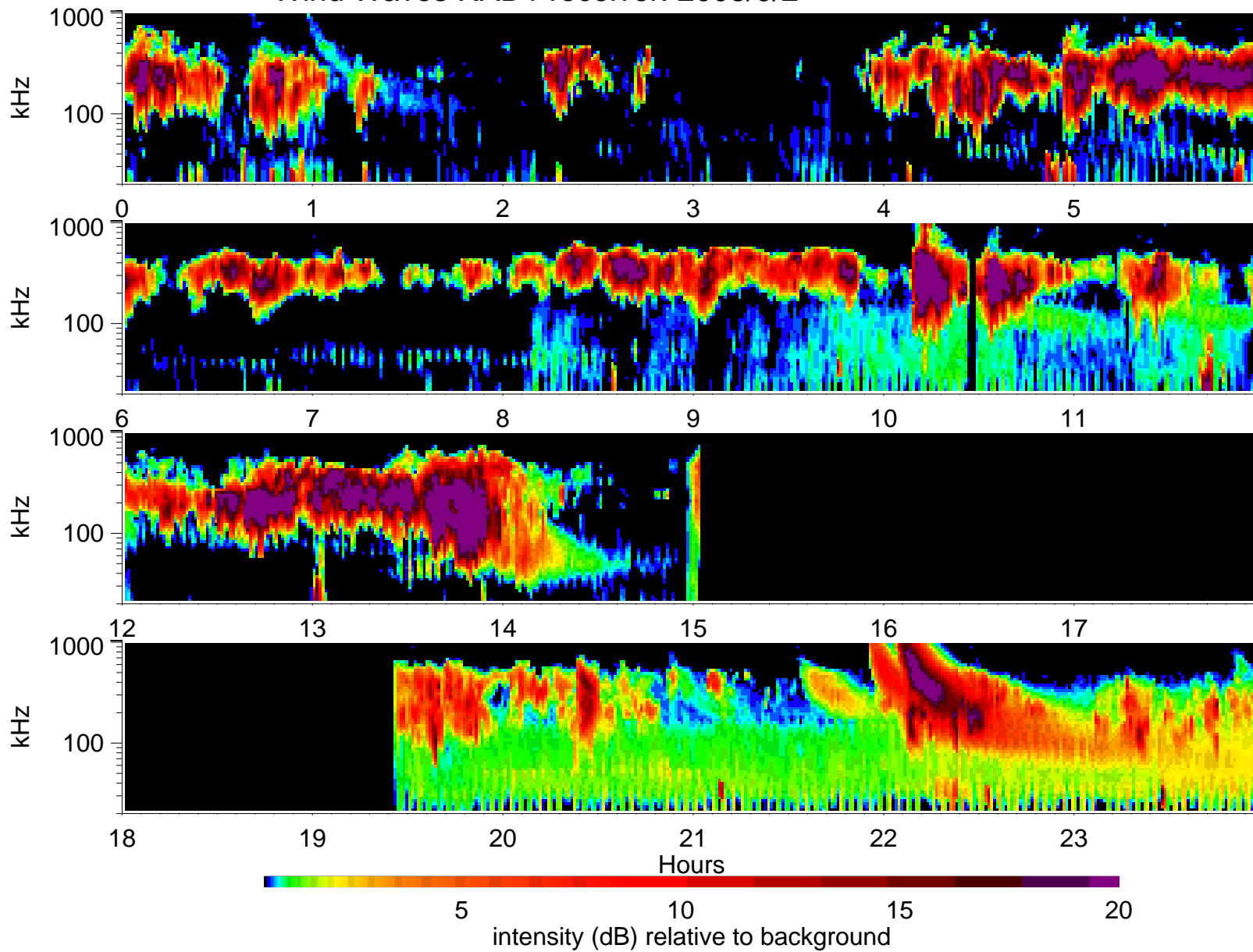
Wind Waves RAD1 receiver: 2003/9/2
