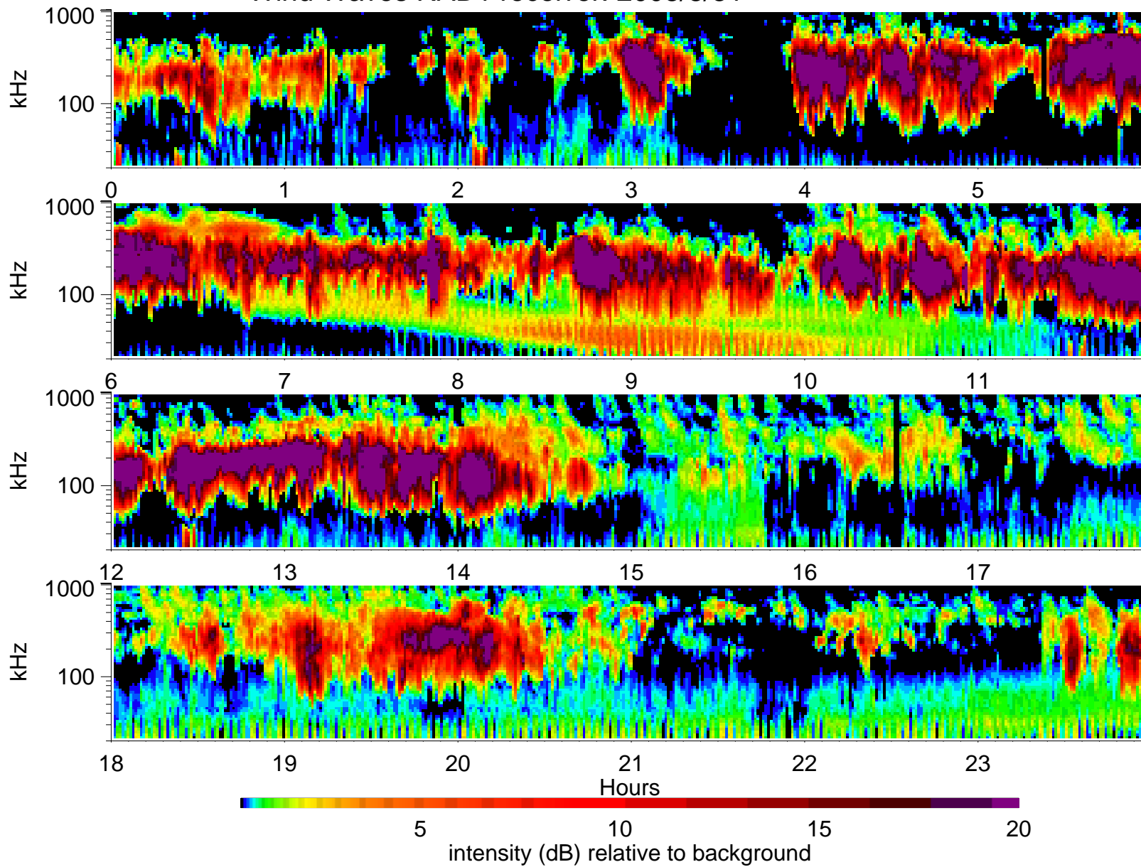
Wind Waves RAD1 receiver: 2003/8/31
