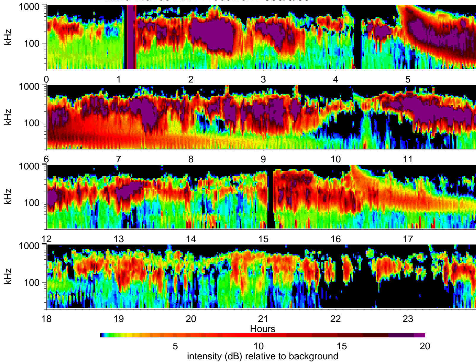
Wind Waves RAD1 receiver: 2003/8/30
