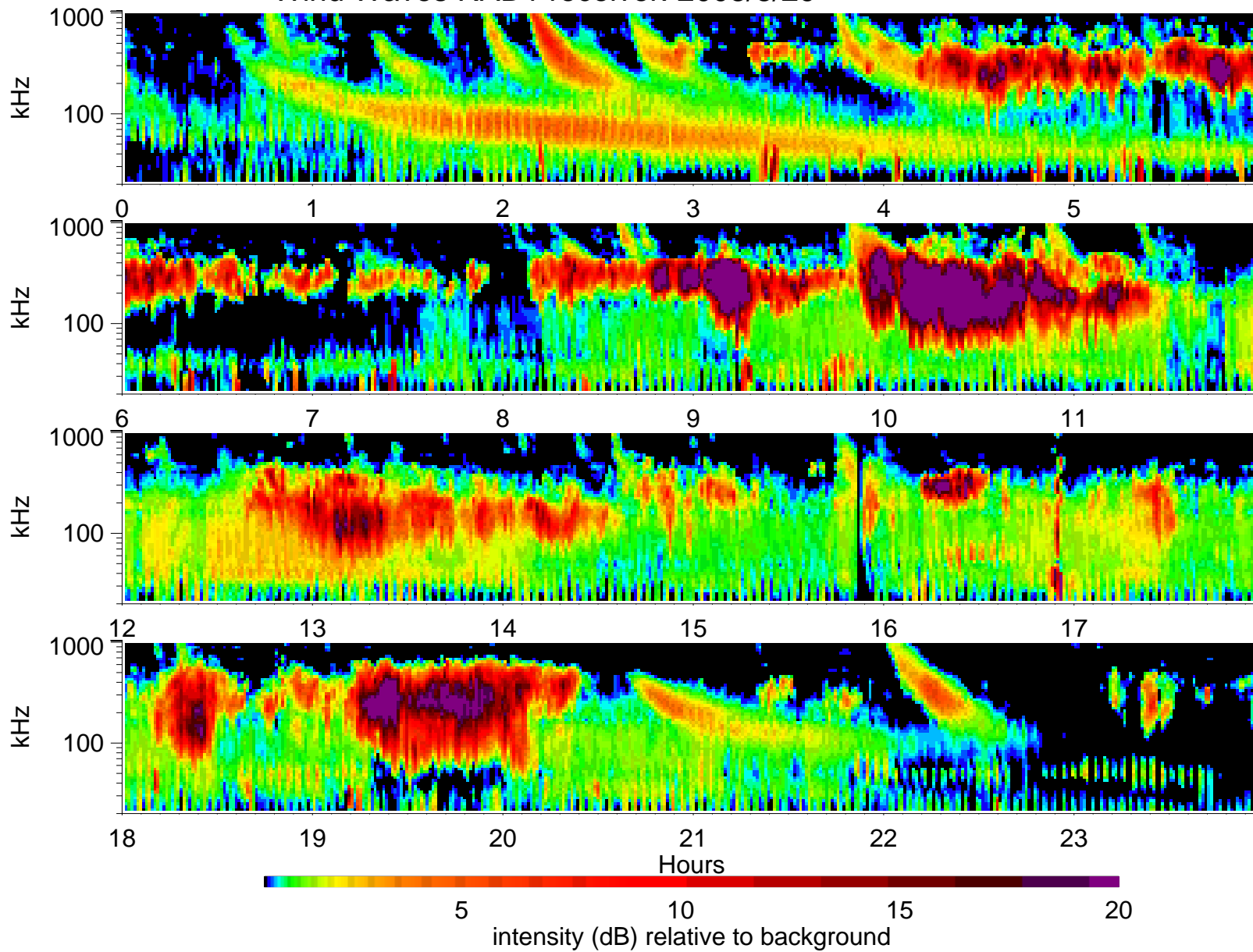
Wind Waves RAD1 receiver: 2003/8/29
