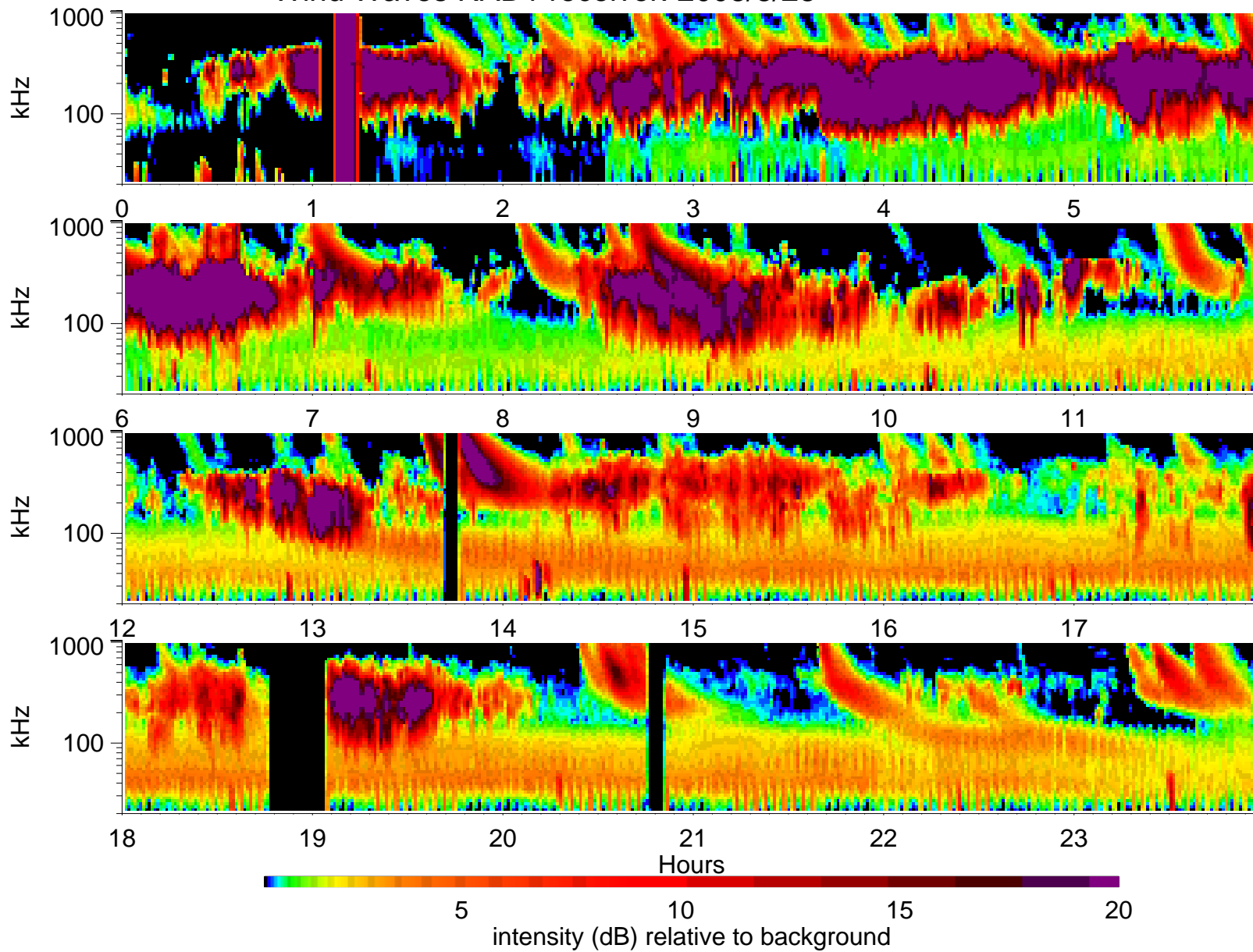
Wind Waves RAD1 receiver: 2003/8/28
