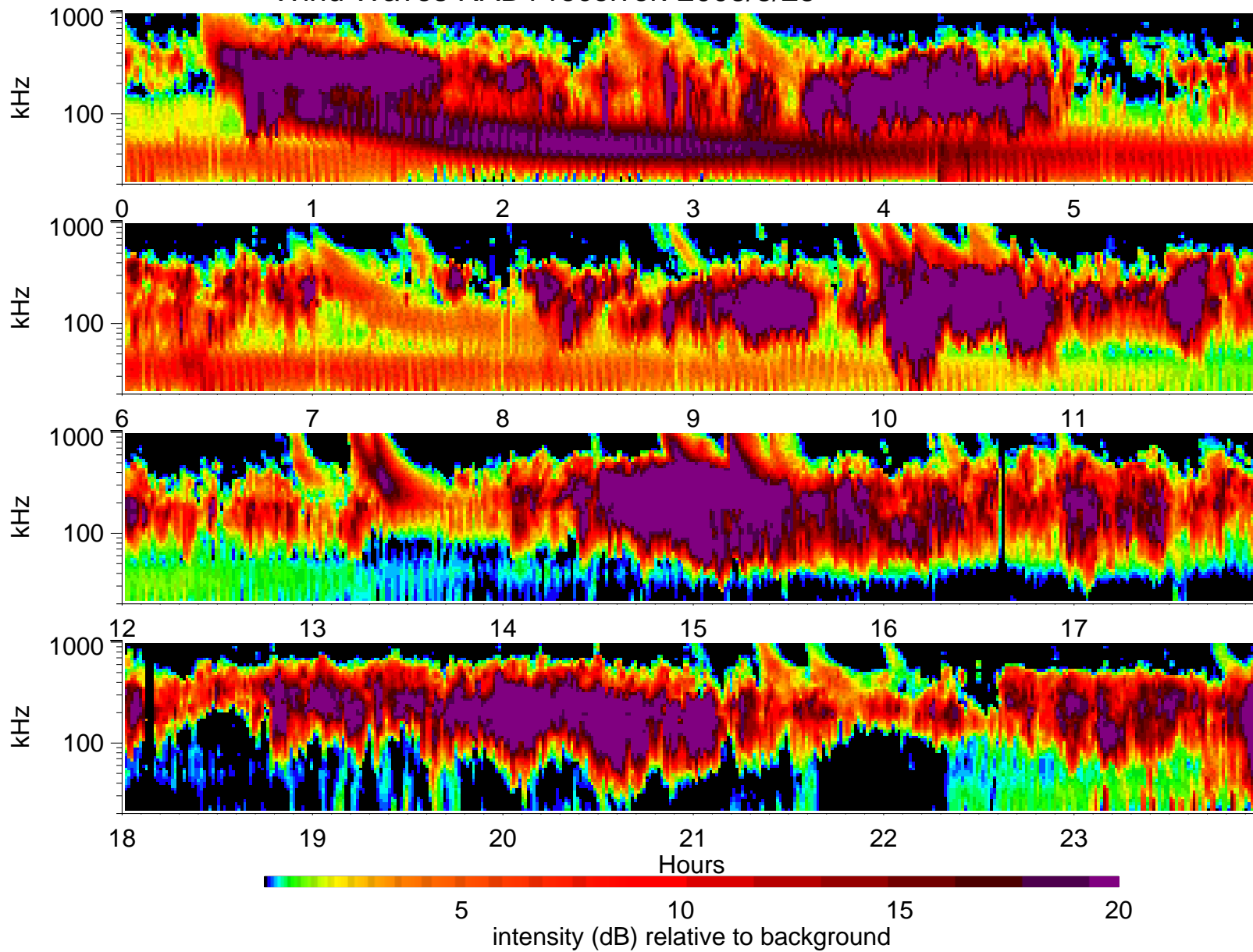
Wind Waves RAD1 receiver: 2003/8/25
