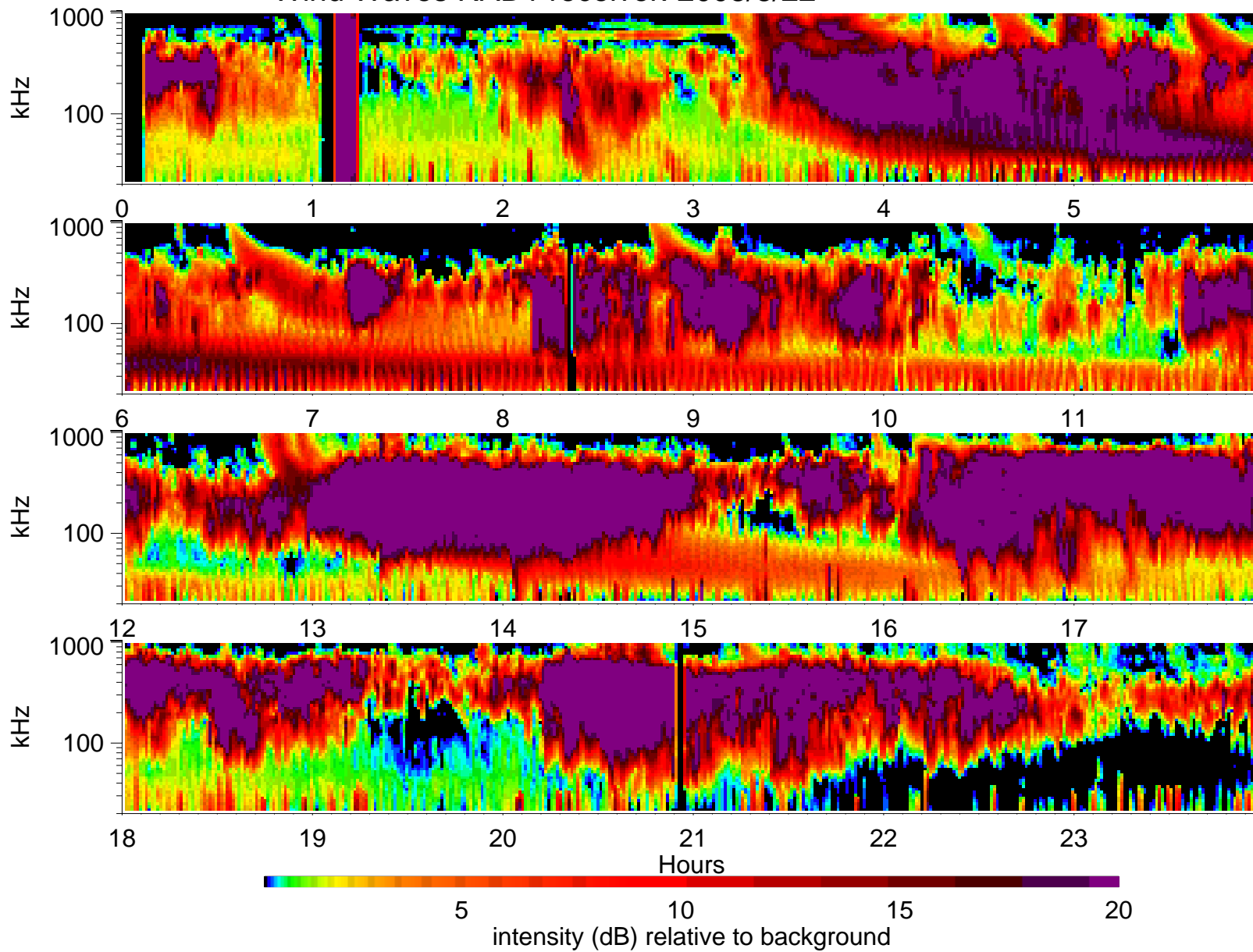
Wind Waves RAD1 receiver: 2003/8/22
