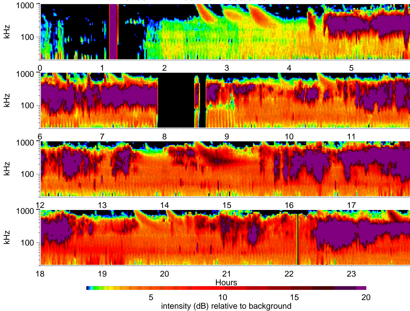
Wind Waves RAD1 receiver: 2003/8/20
