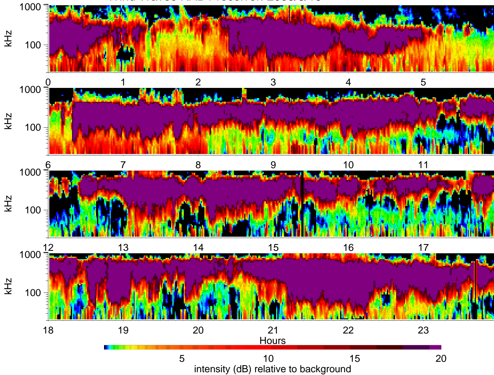
Wind Waves RAD1 receiver: 2003/8/13
