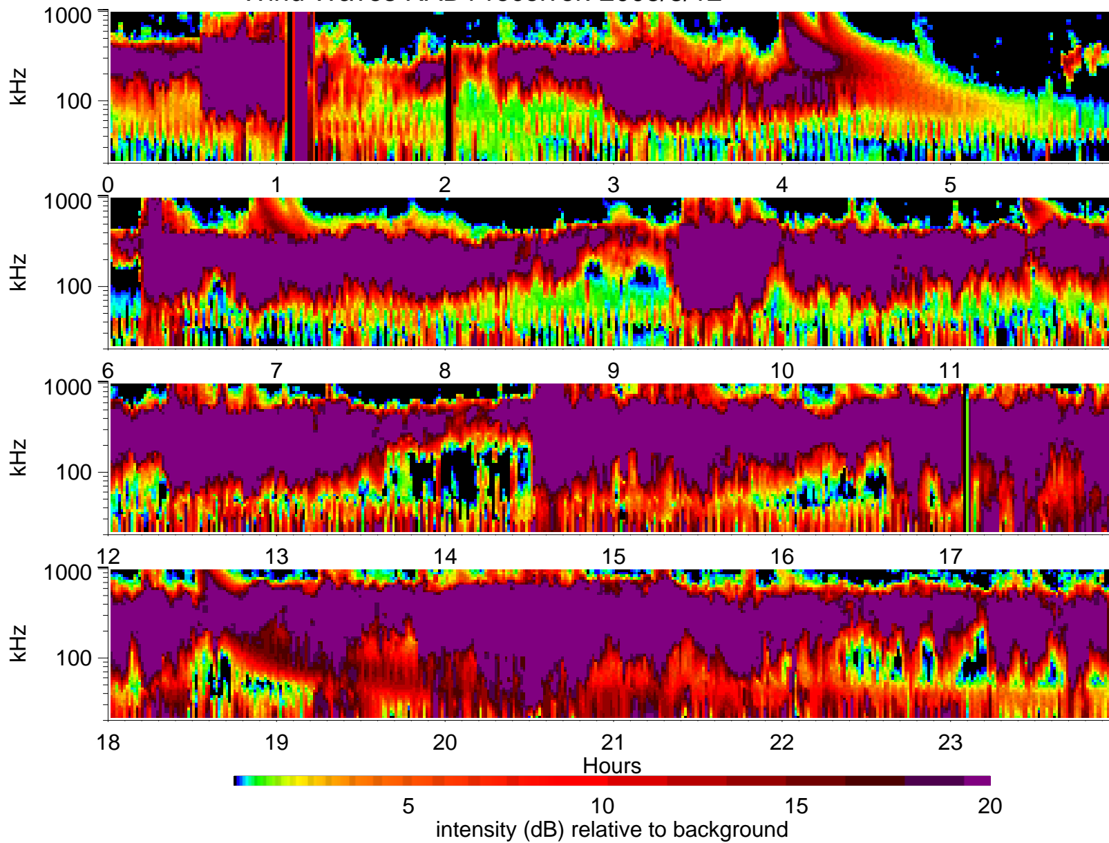
Wind Waves RAD1 receiver: 2003/8/12
