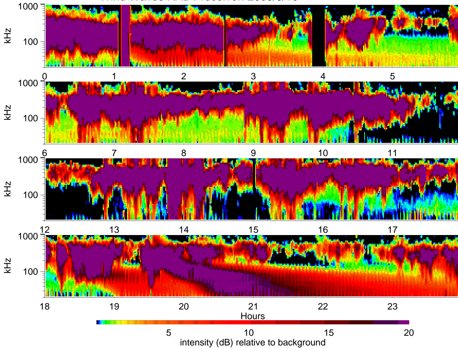
Wind Waves RAD1 receiver: 2003/8/10
