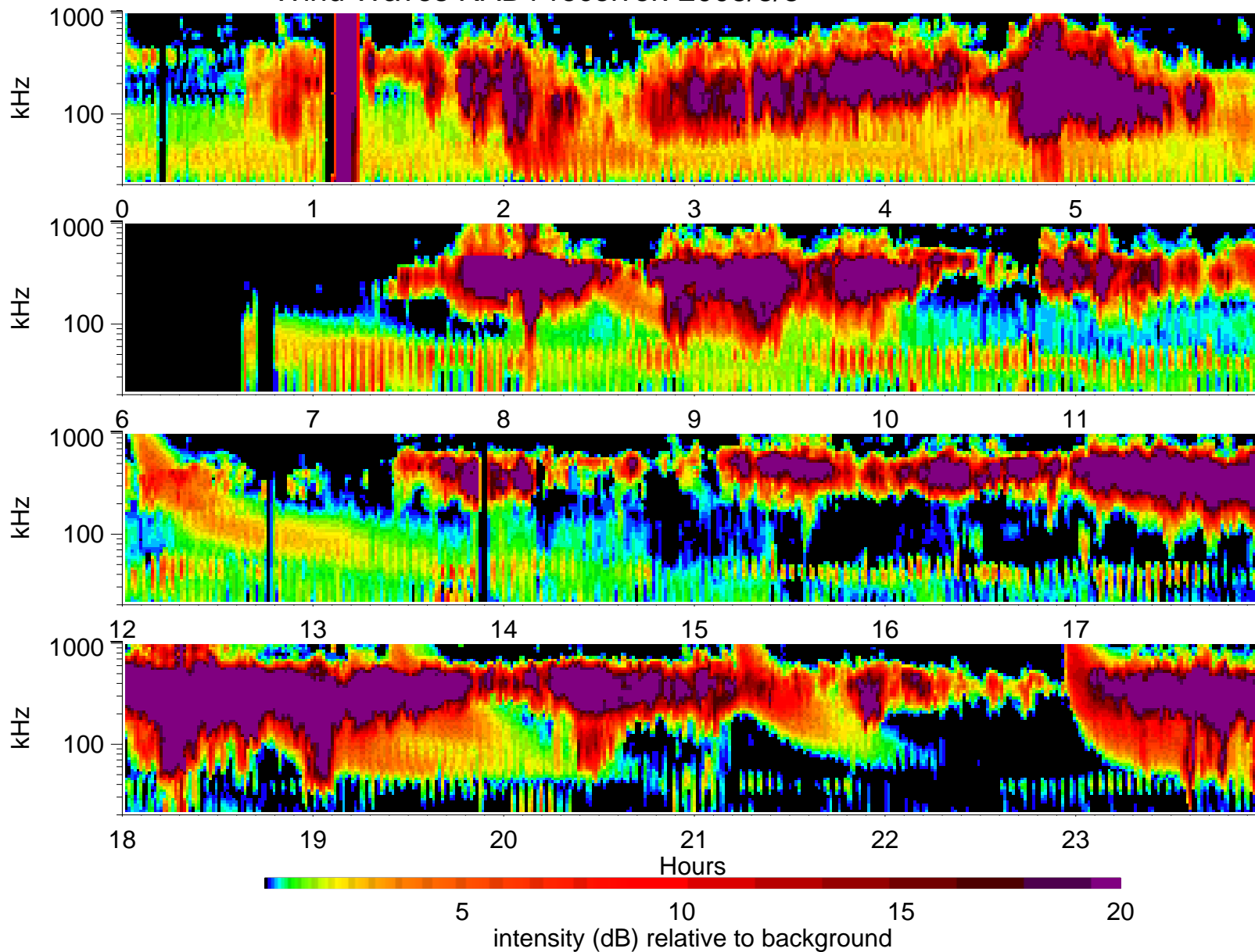
Wind Waves RAD1 receiver: 2003/8/8
