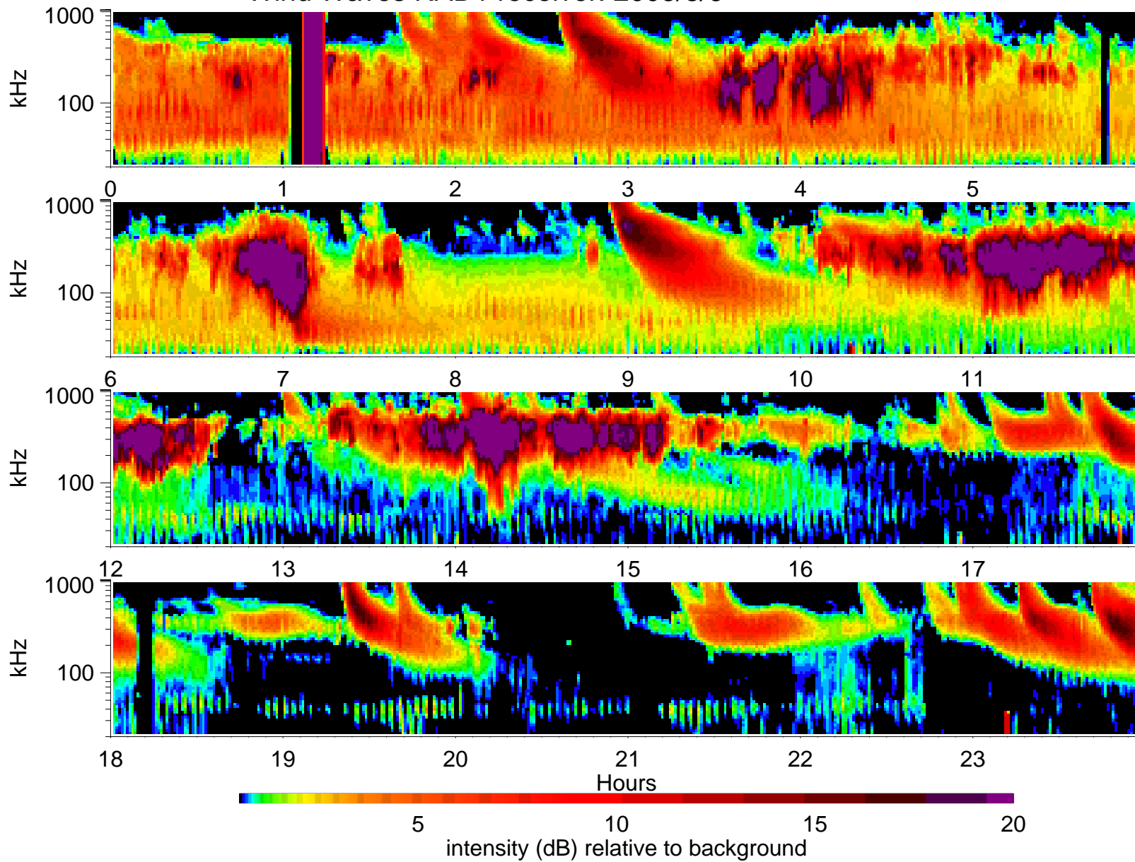
Wind Waves RAD1 receiver: 2003/8/6
