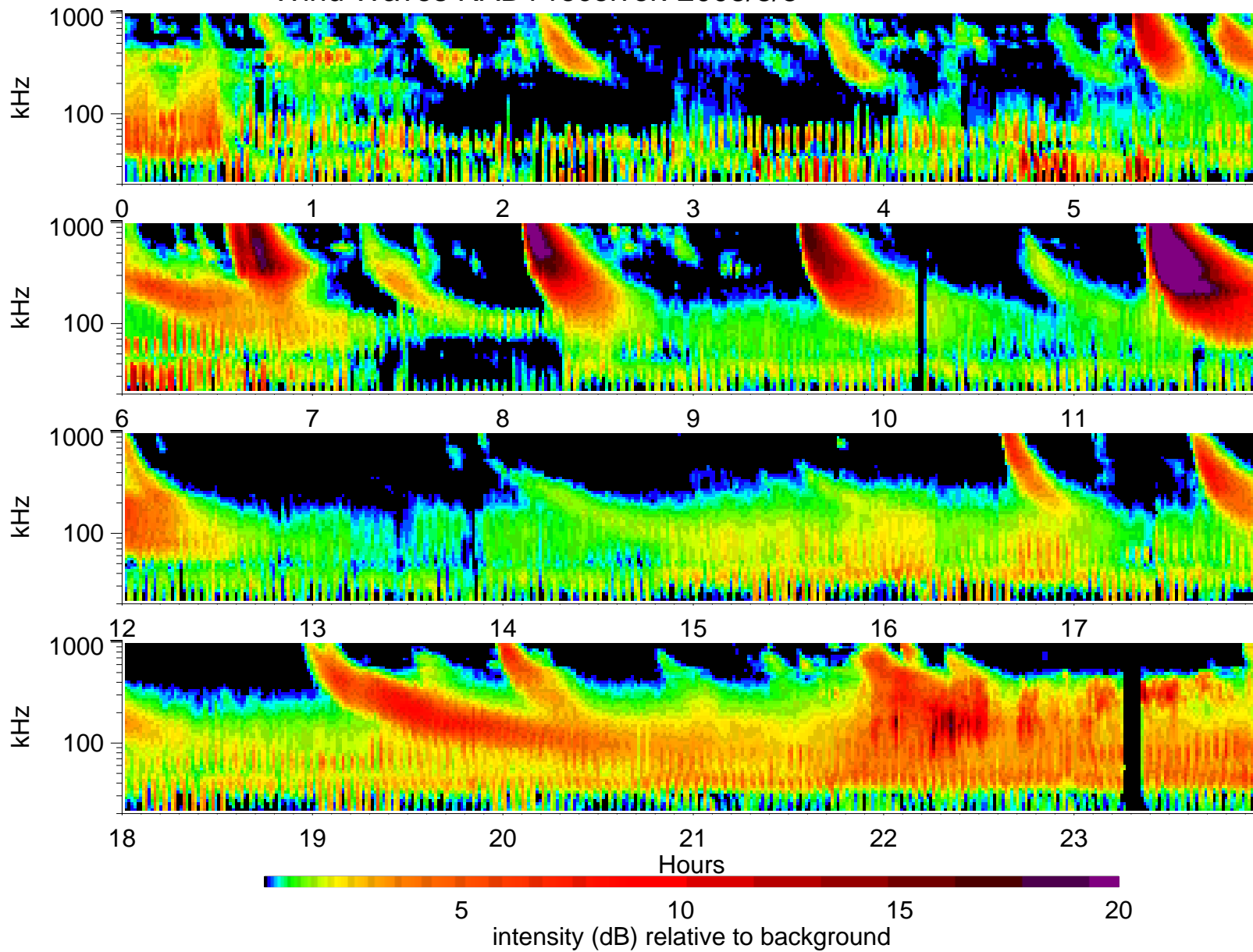
Wind Waves RAD1 receiver: 2003/8/5
