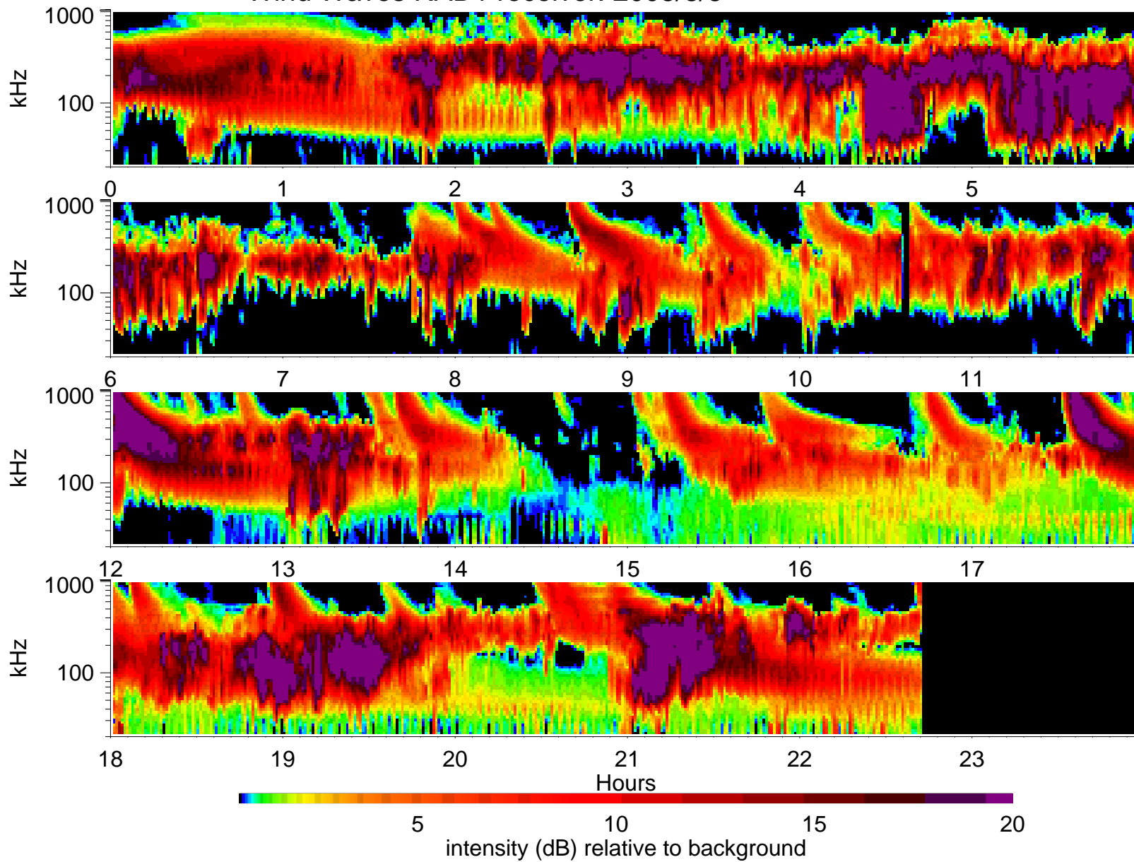
Wind Waves RAD1 receiver: 2003/8/3
