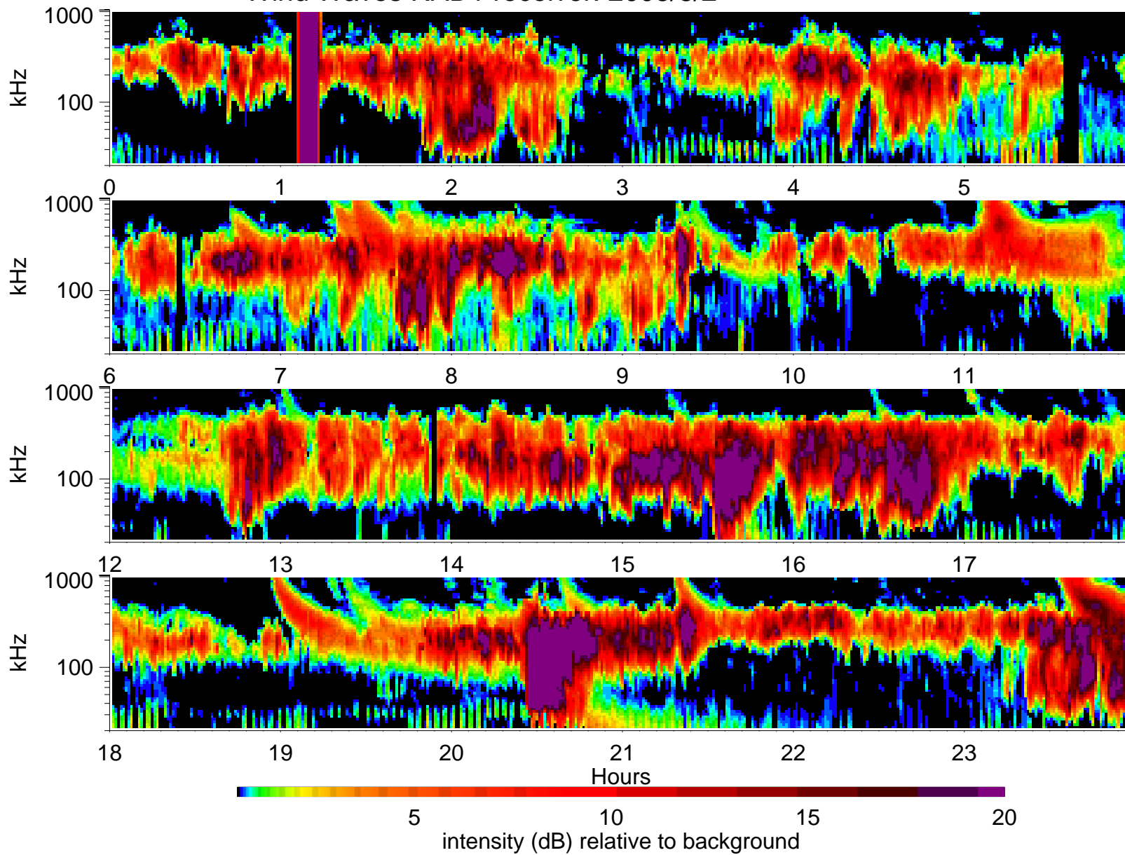
Wind Waves RAD1 receiver: 2003/8/2
