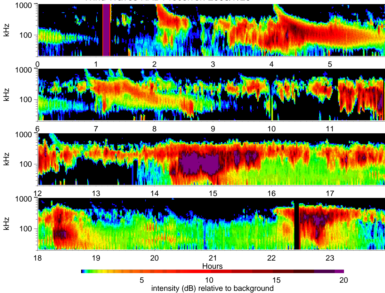
Wind Waves RAD1 receiver: 2003/7/29
