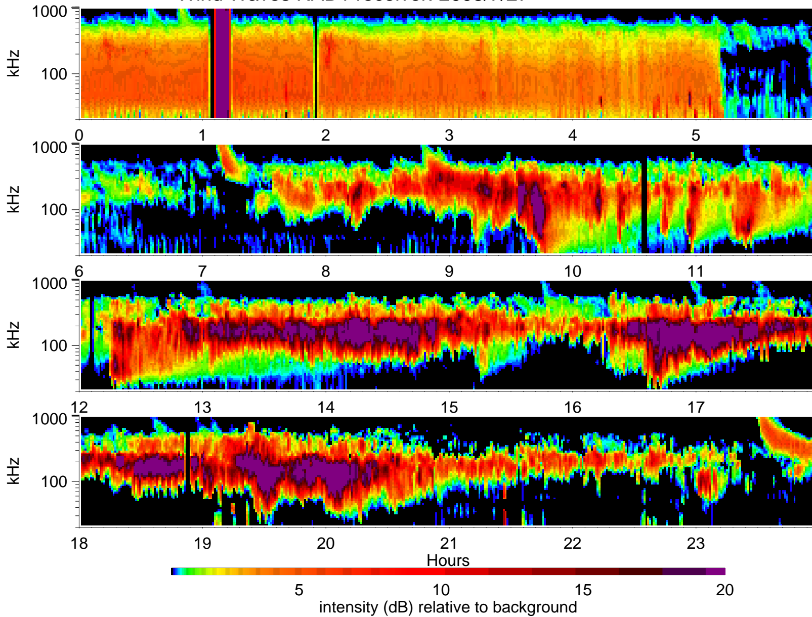
Wind Waves RAD1 receiver: 2003/7/27
