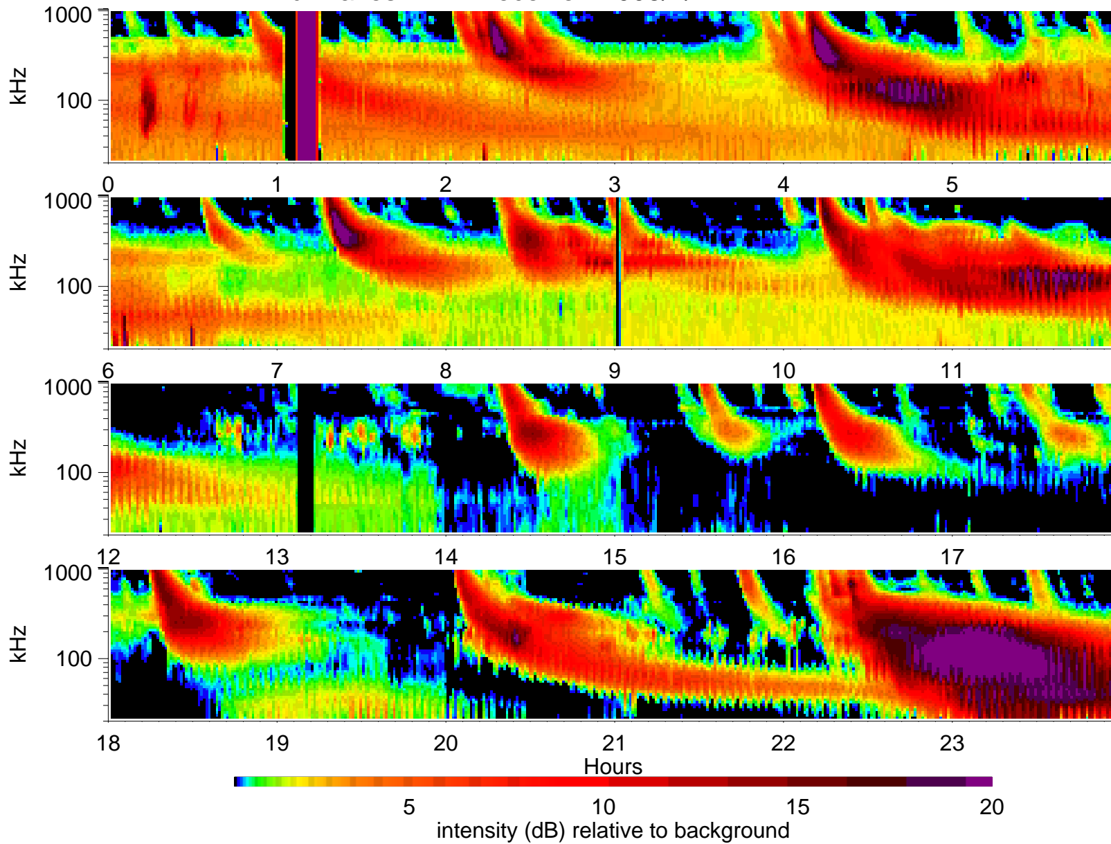
Wind Waves RAD1 receiver: 2003/7/21
