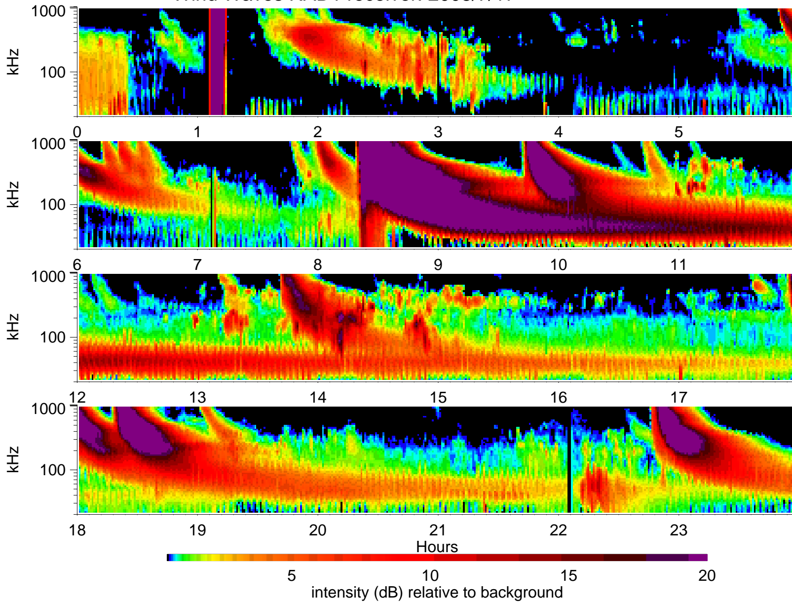
Wind Waves RAD1 receiver: 2003/7/17
