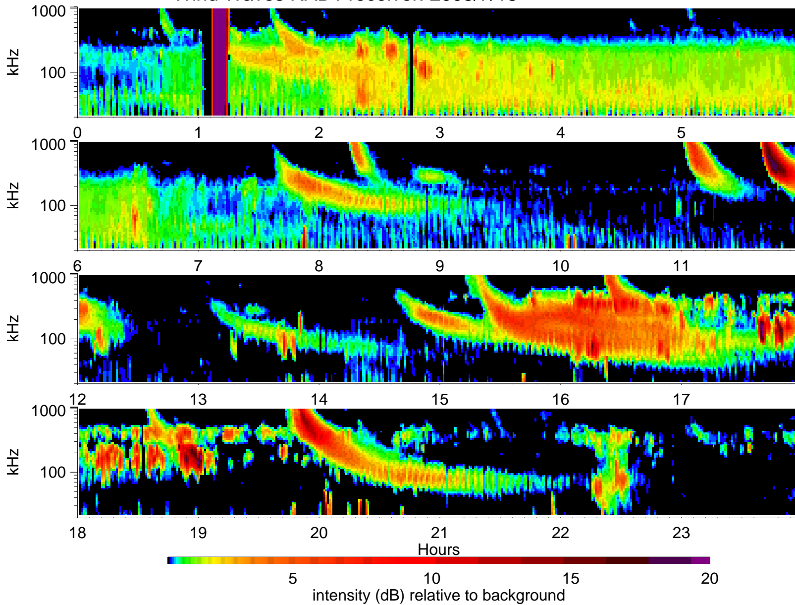
Wind Waves RAD1 receiver: 2003/7/13
