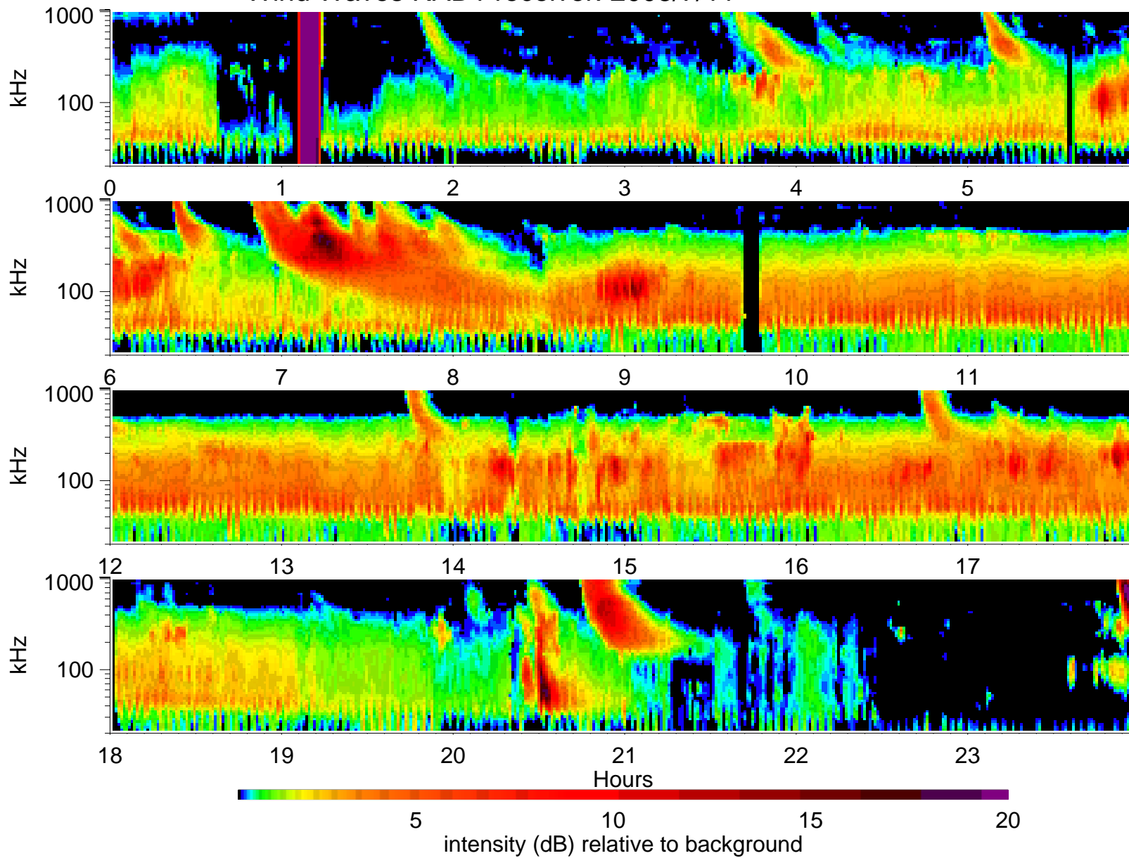
Wind Waves RAD1 receiver: 2003/7/11
