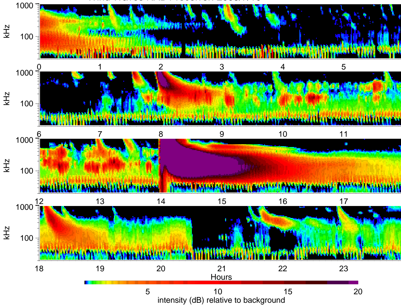
Wind Waves RAD1 receiver: 2003/7/10
