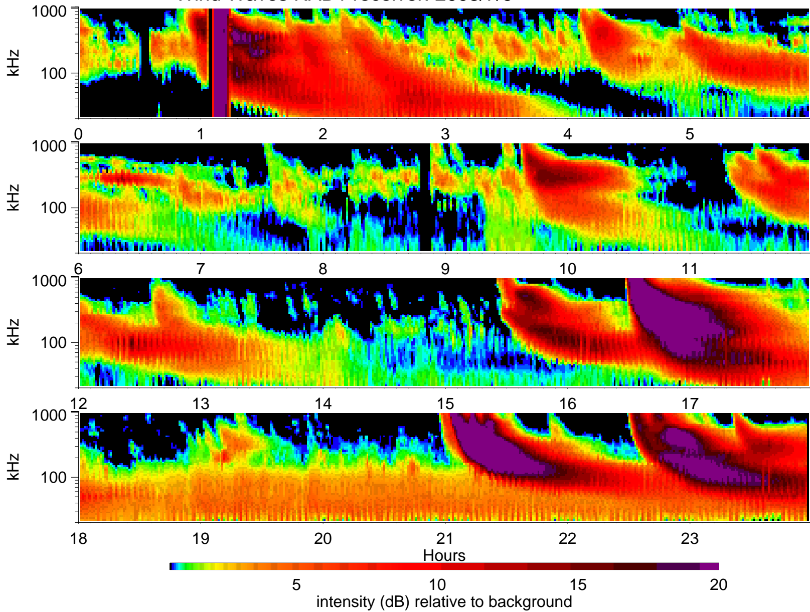
Wind Waves RAD1 receiver: 2003/7/9
