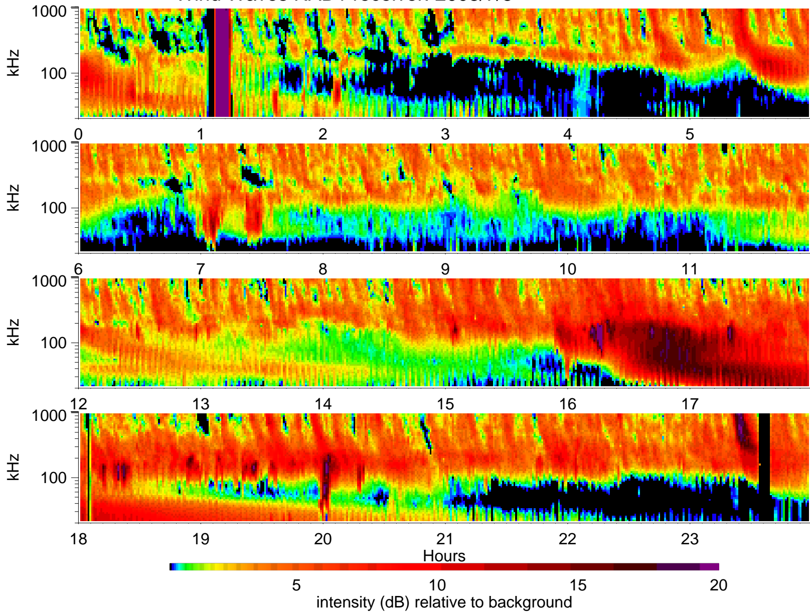
Wind Waves RAD1 receiver: 2003/7/5
