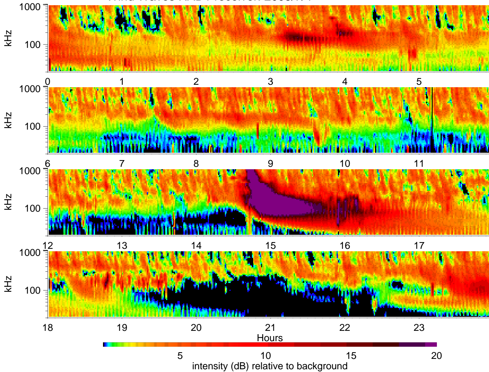
Wind Waves RAD1 receiver: 2003/7/4
