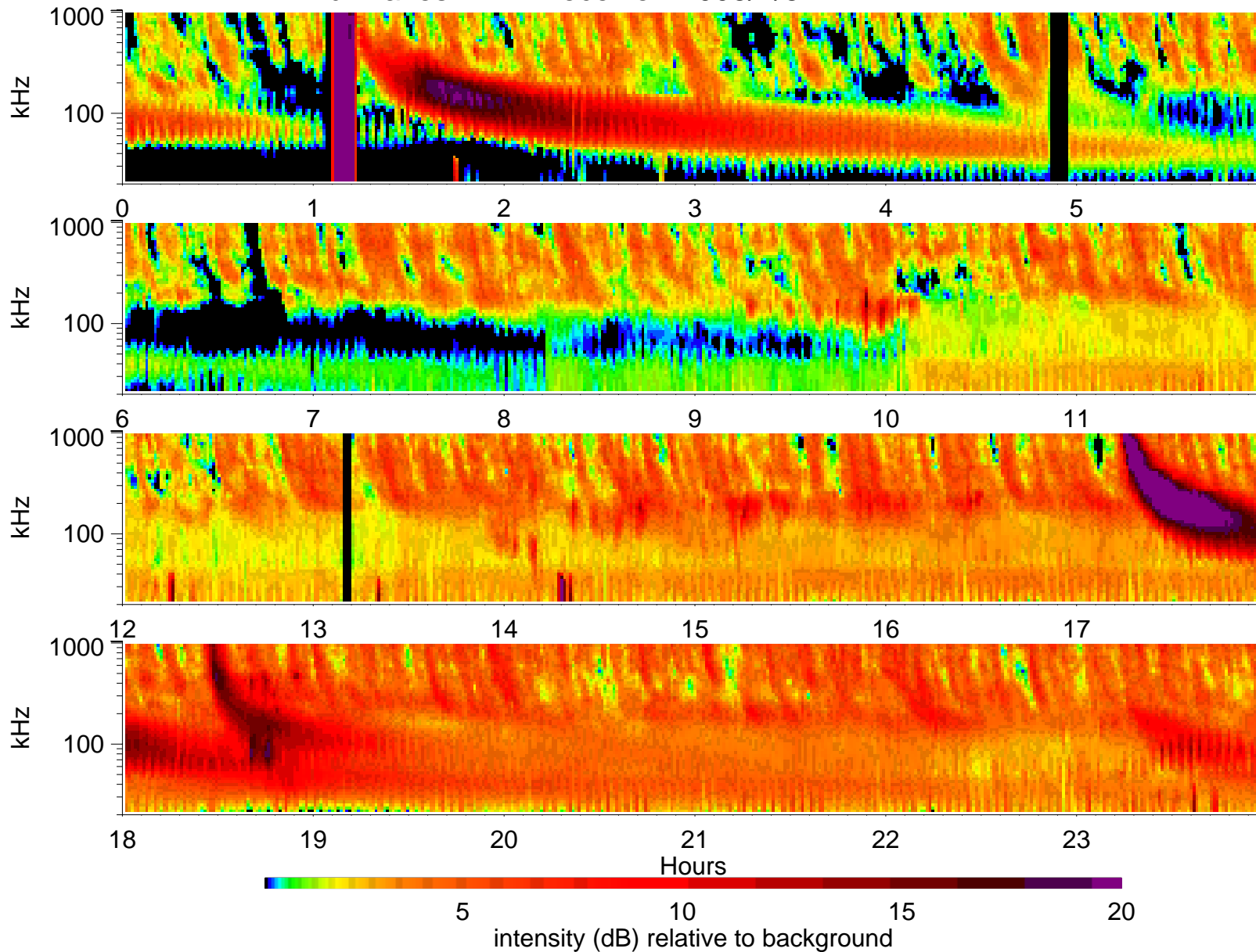
Wind Waves RAD1 receiver: 2003/7/3
