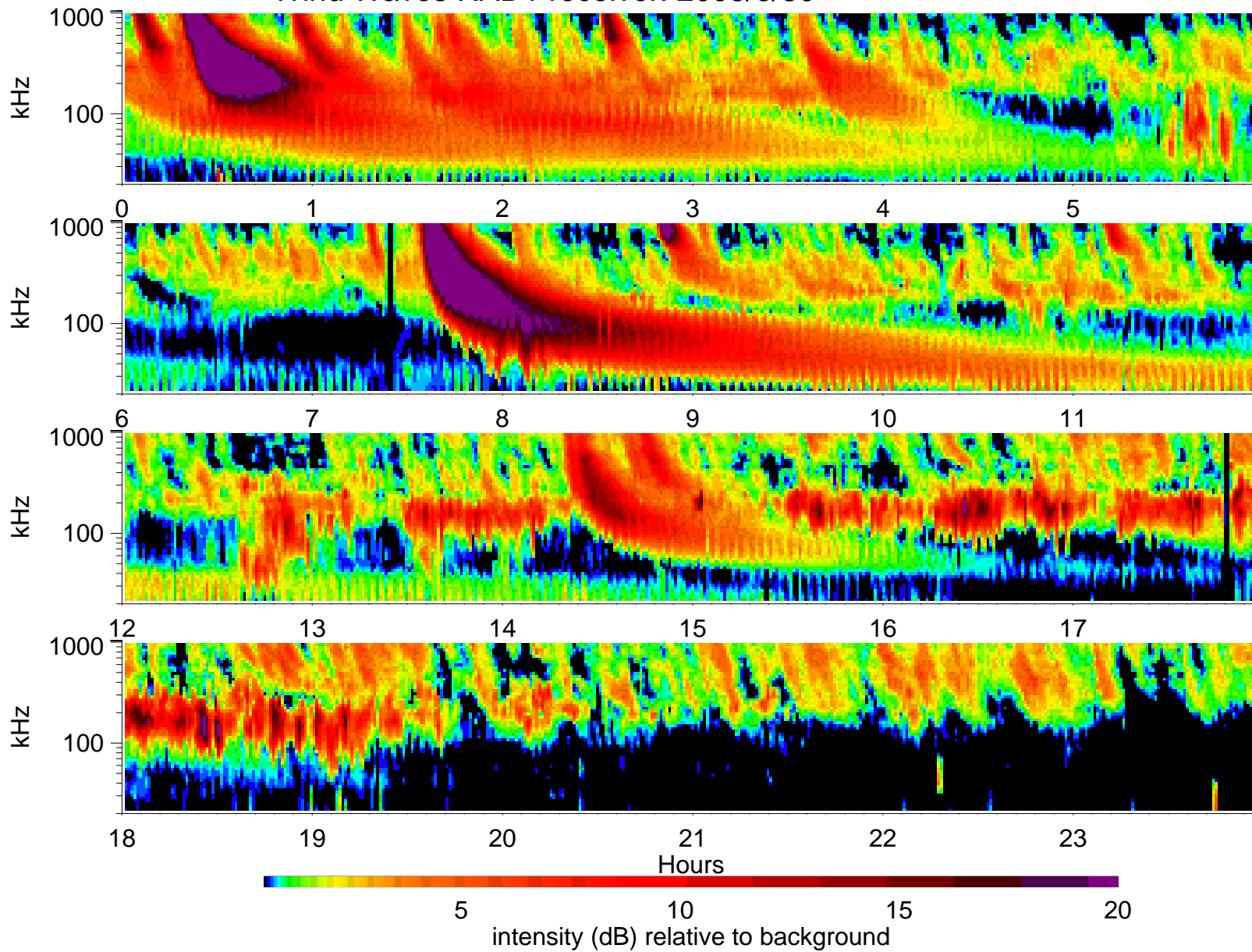
Wind Waves RAD1 receiver: 2003/6/30
