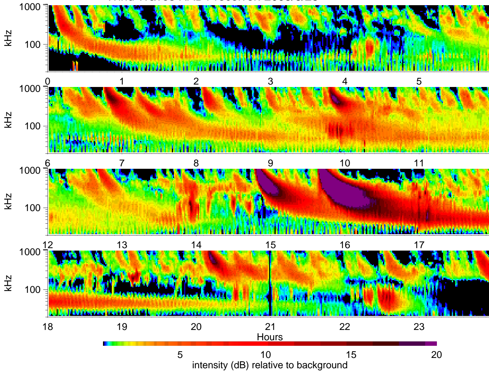
Wind Waves RAD1 receiver: 2003/6/28
