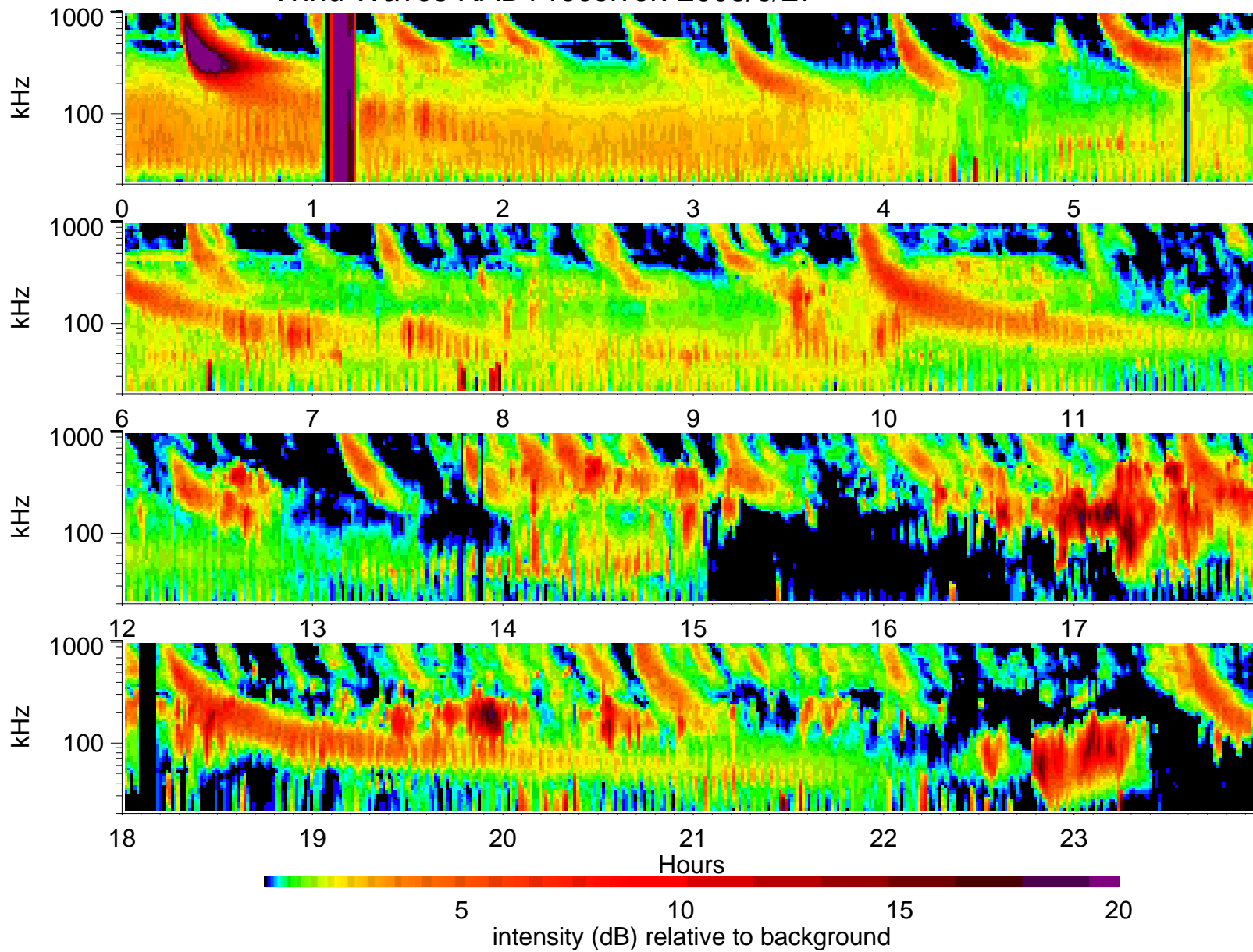
Wind Waves RAD1 receiver: 2003/6/27
