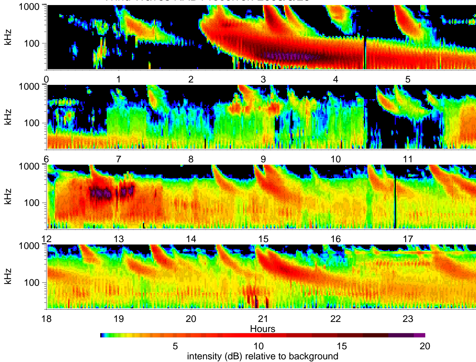
Wind Waves RAD1 receiver: 2003/6/26
