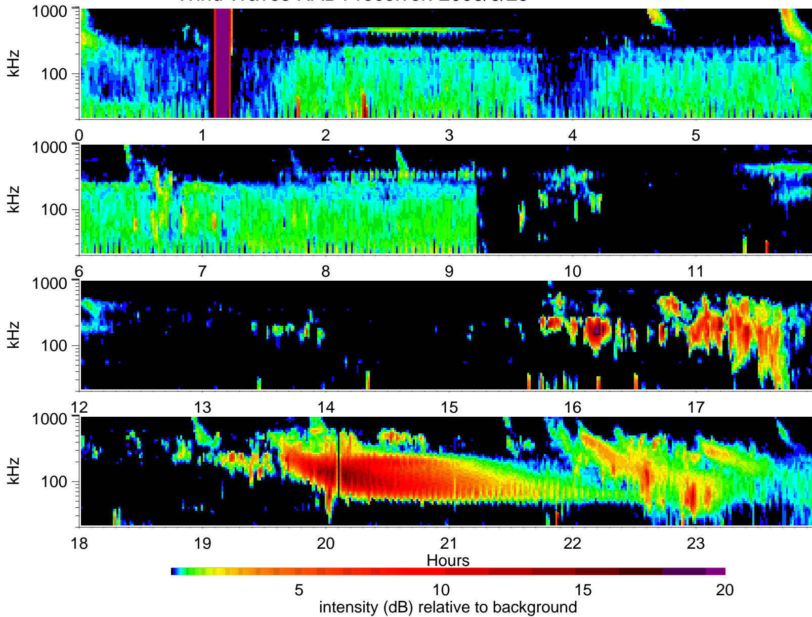
Wind Waves RAD1 receiver: 2003/6/25
