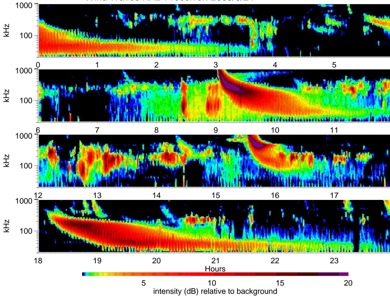
Wind Waves RAD1 receiver: 2003/6/24
