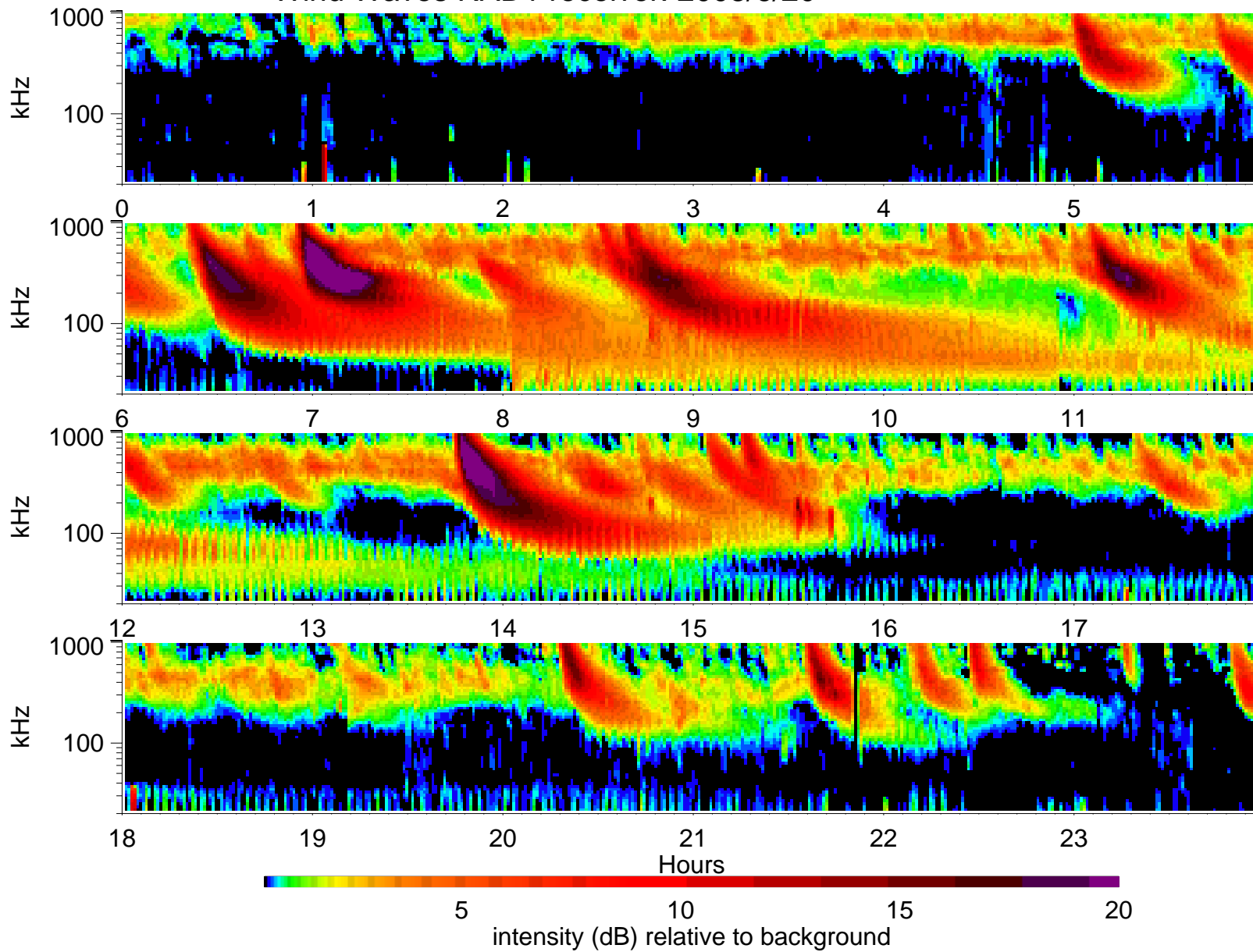
Wind Waves RAD1 receiver: 2003/6/20
