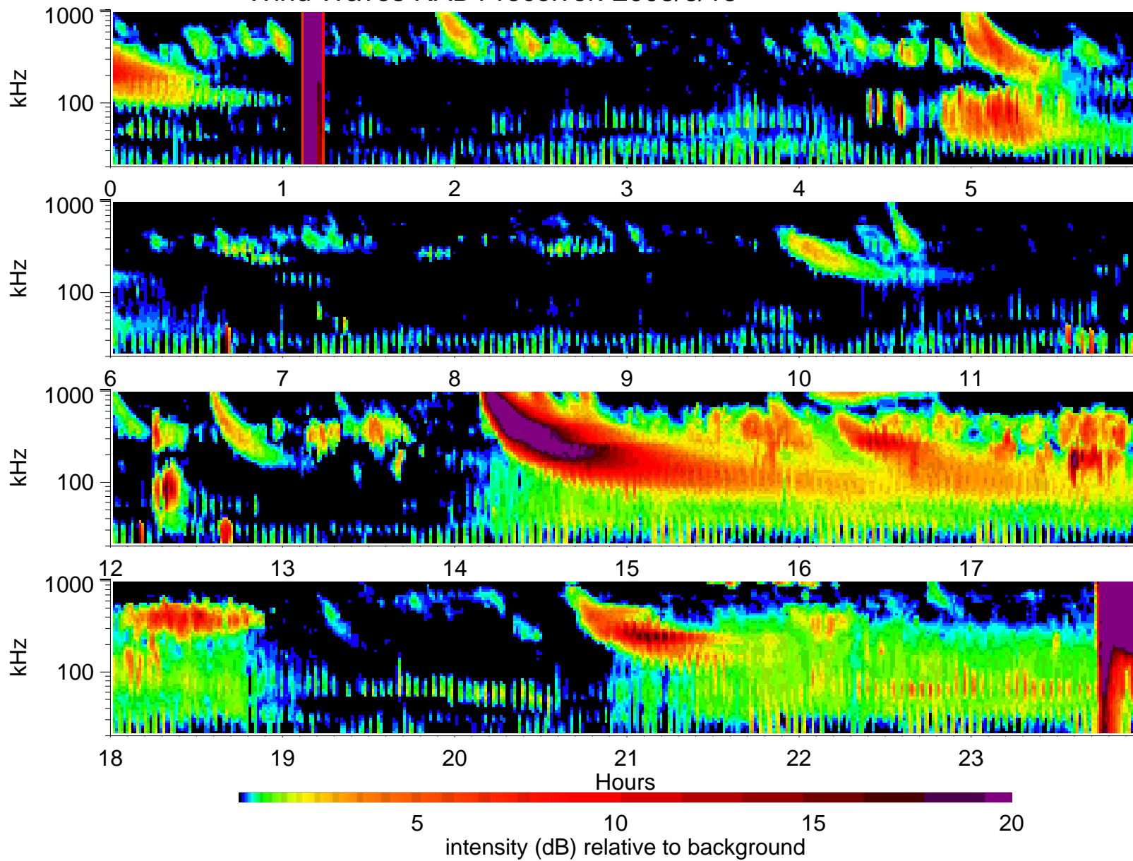
Wind Waves RAD1 receiver: 2003/6/15
