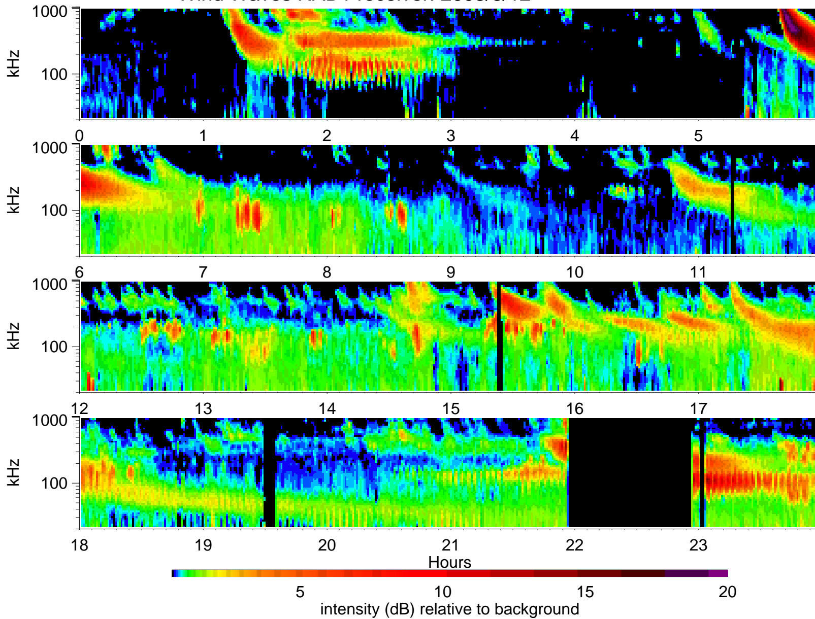
Wind Waves RAD1 receiver: 2003/6/12
