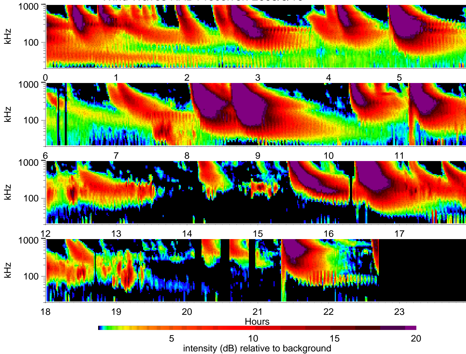
Wind Waves RAD1 receiver: 2003/6/10
