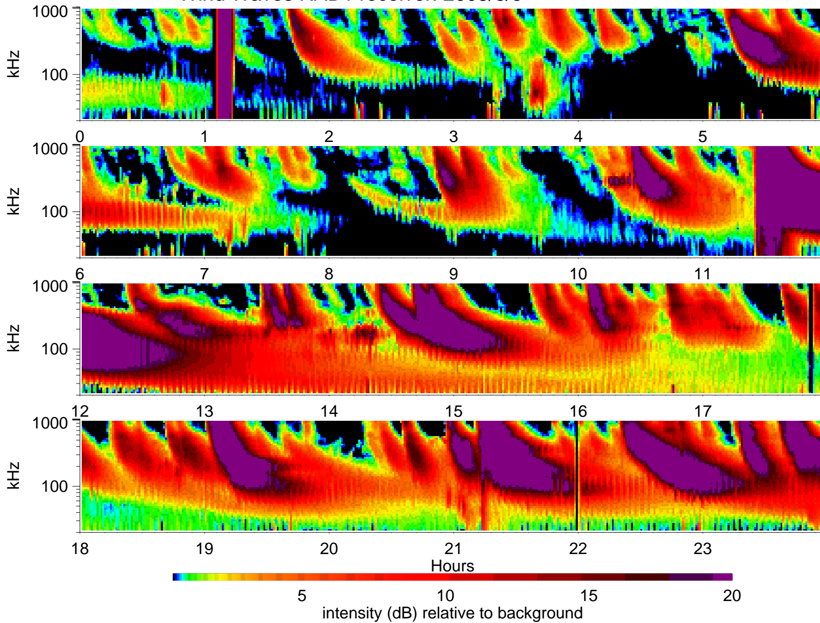
Wind Waves RAD1 receiver: 2003/6/9
