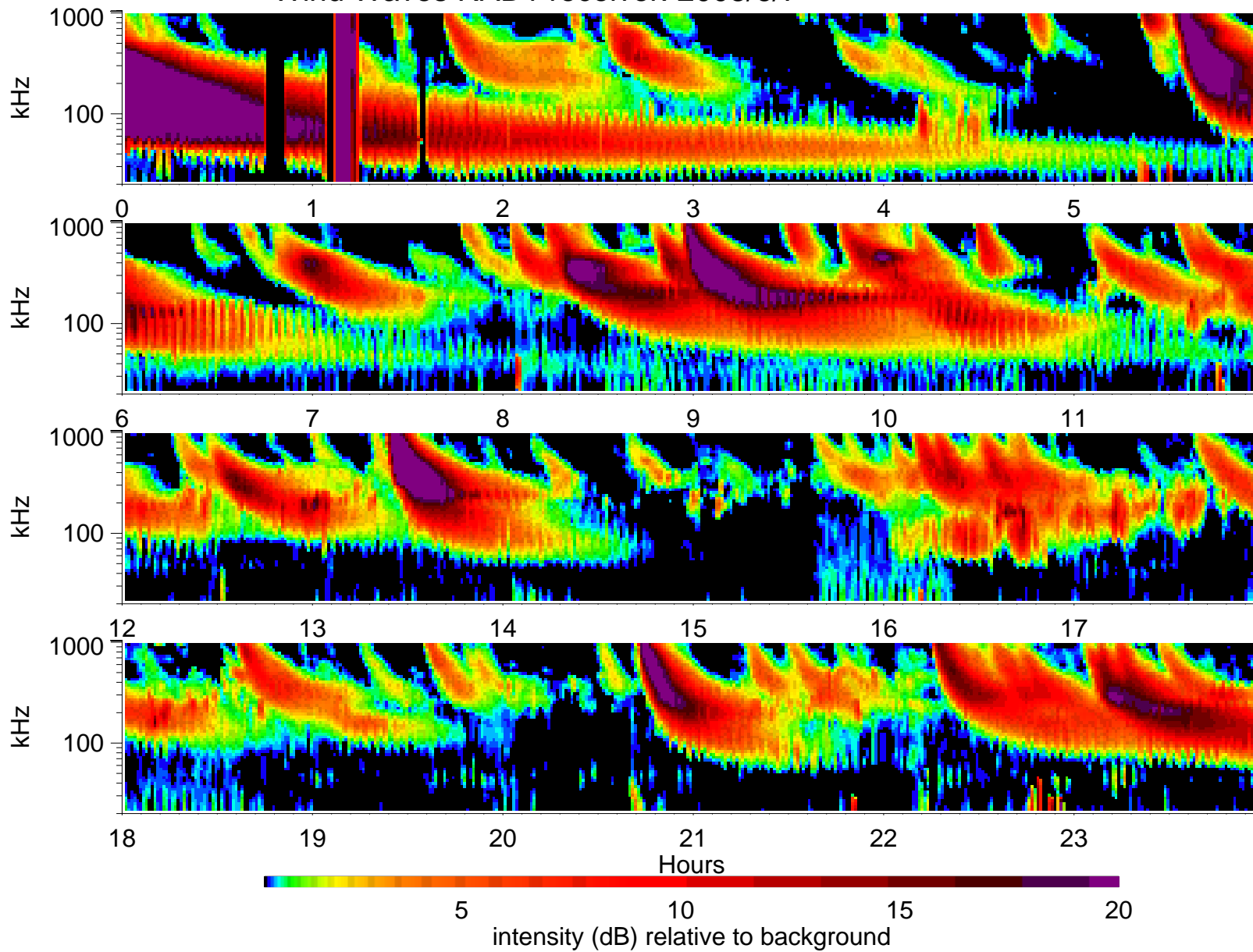
Wind Waves RAD1 receiver: 2003/6/7
