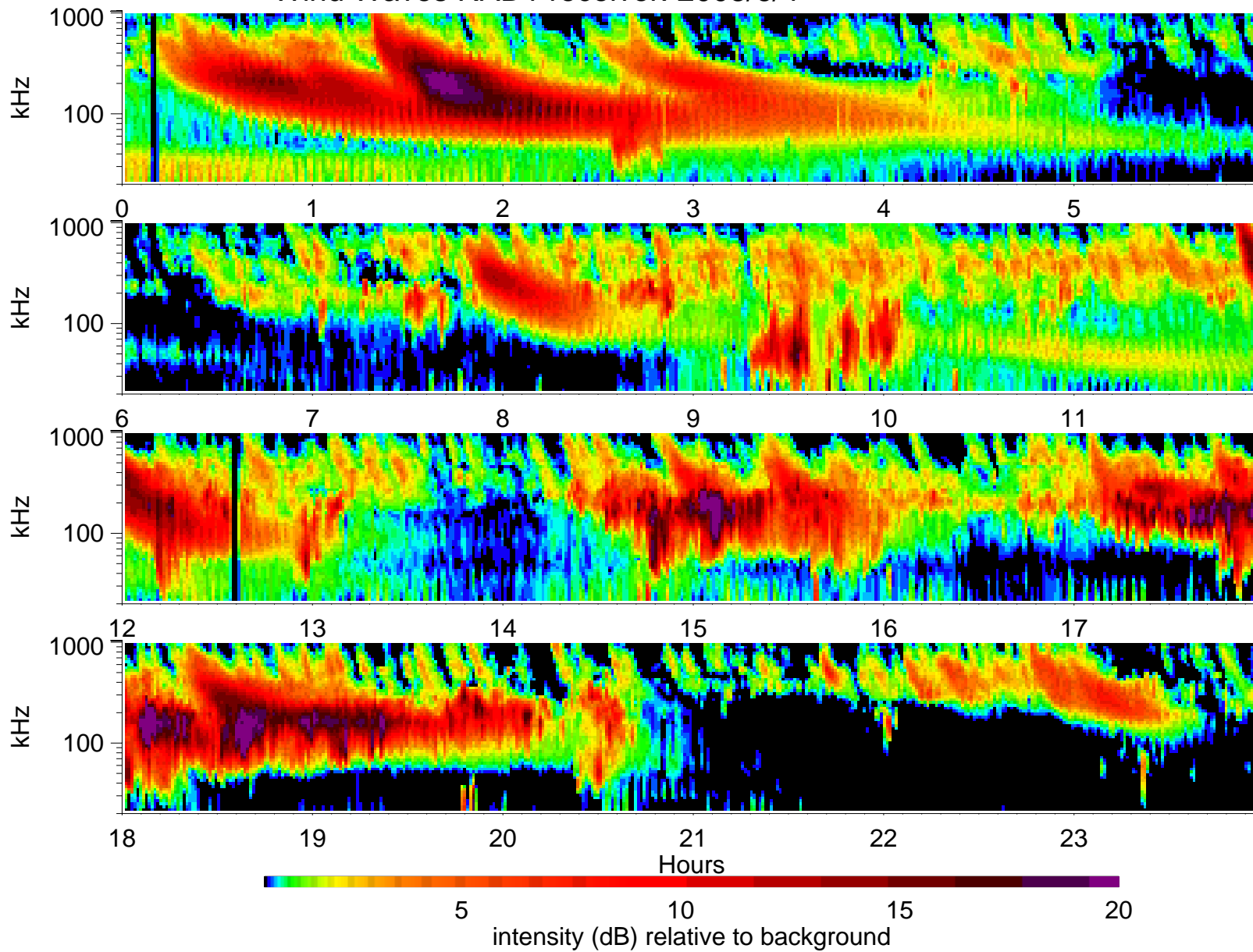
Wind Waves RAD1 receiver: 2003/6/4
