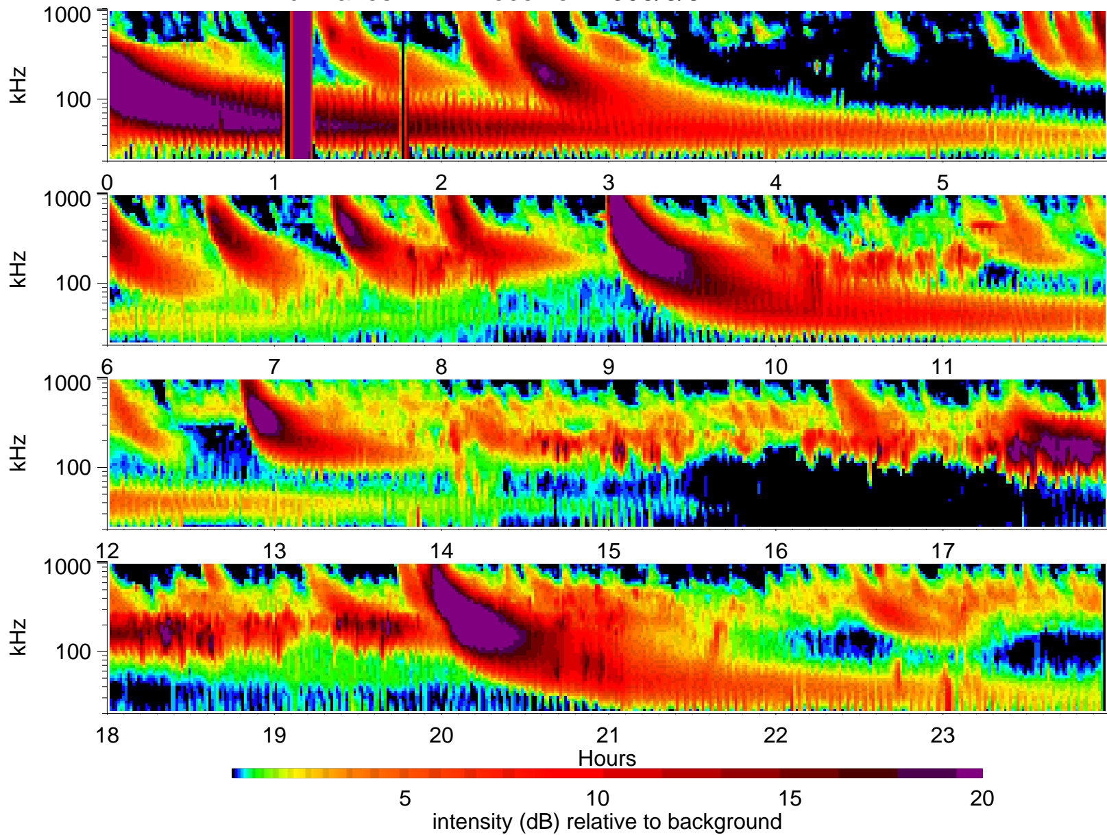
Wind Waves RAD1 receiver: 2003/6/3
