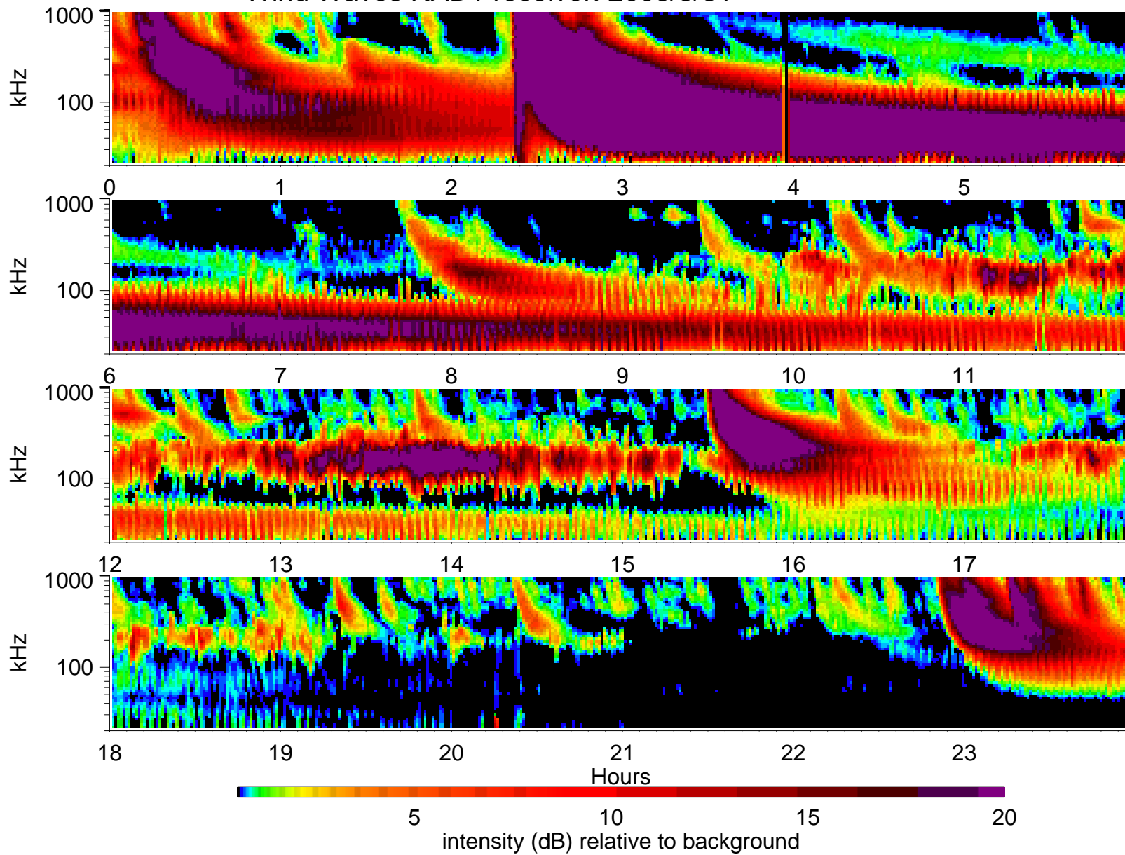
Wind Waves RAD1 receiver: 2003/5/31
