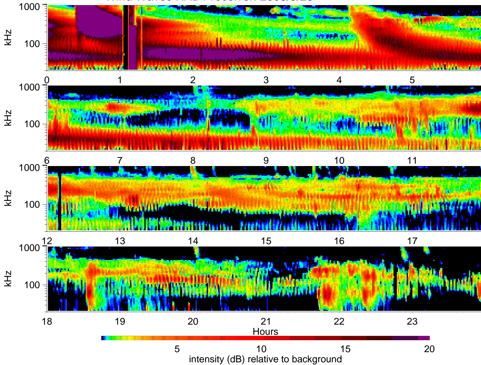
Wind Waves RAD1 receiver: 2003/5/28
